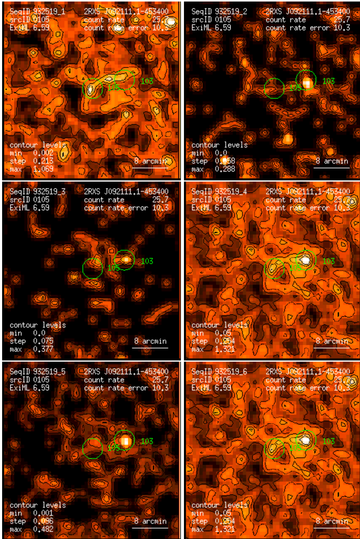
Figure 105: RASS 932519: detection 0105: band rate images, Gaussian filter: (1) PSPC channels 11 – 41, (2) 52 – 90, (3) 91 – 201, (4) 11 – 235, (5) 52 – 201, (6) 11 – 201. Broad band rates in counts/ks. Band rate contour levels in counts/ks/arcmin 2 .
