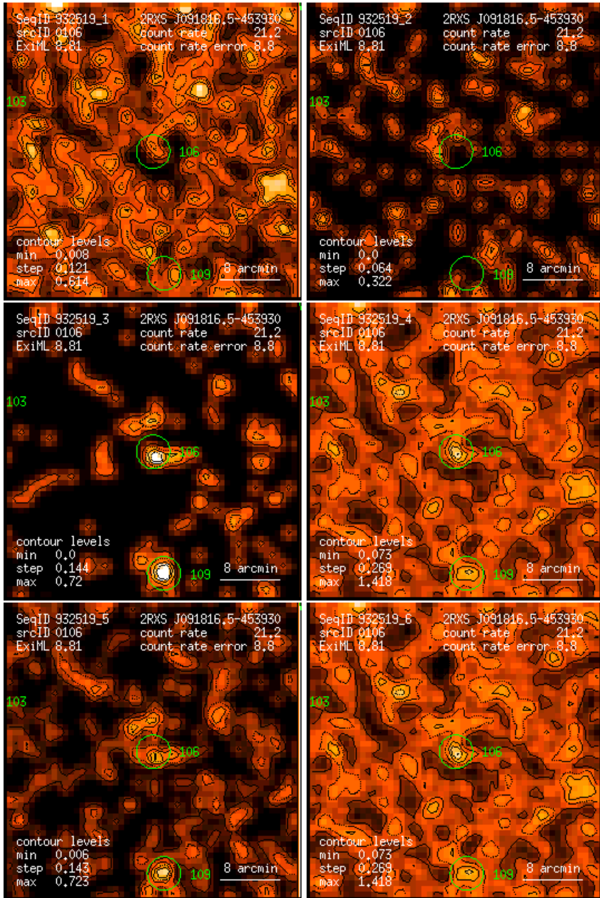
Figure 106: RASS 932519: detection 0106: band rate images, Gaussian filter: (1) PSPC channels 11 – 41, (2) 52 – 90, (3) 91 – 201, (4) 11 – 235, (5) 52 – 201, (6) 11 – 201. Broad band rates in counts/ks. Band rate contour levels in counts/ks/arcmin 2 .
