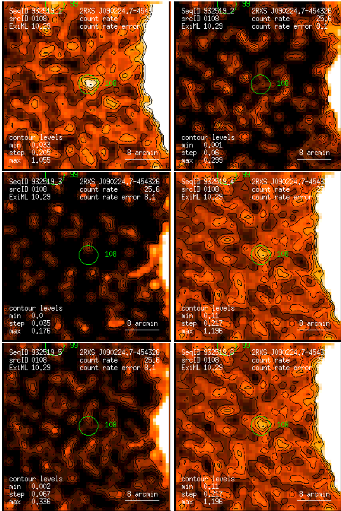
Figure 108: RASS 932519: detection 0108: band rate images, Gaussian filter: (1) PSPC channels 11 – 41, (2) 52 – 90, (3) 91 – 201, (4) 11 – 235, (5) 52 – 201, (6) 11 – 201. Broad band rates in counts/ks. Band rate contour levels in counts/ks/arcmin 2 .
