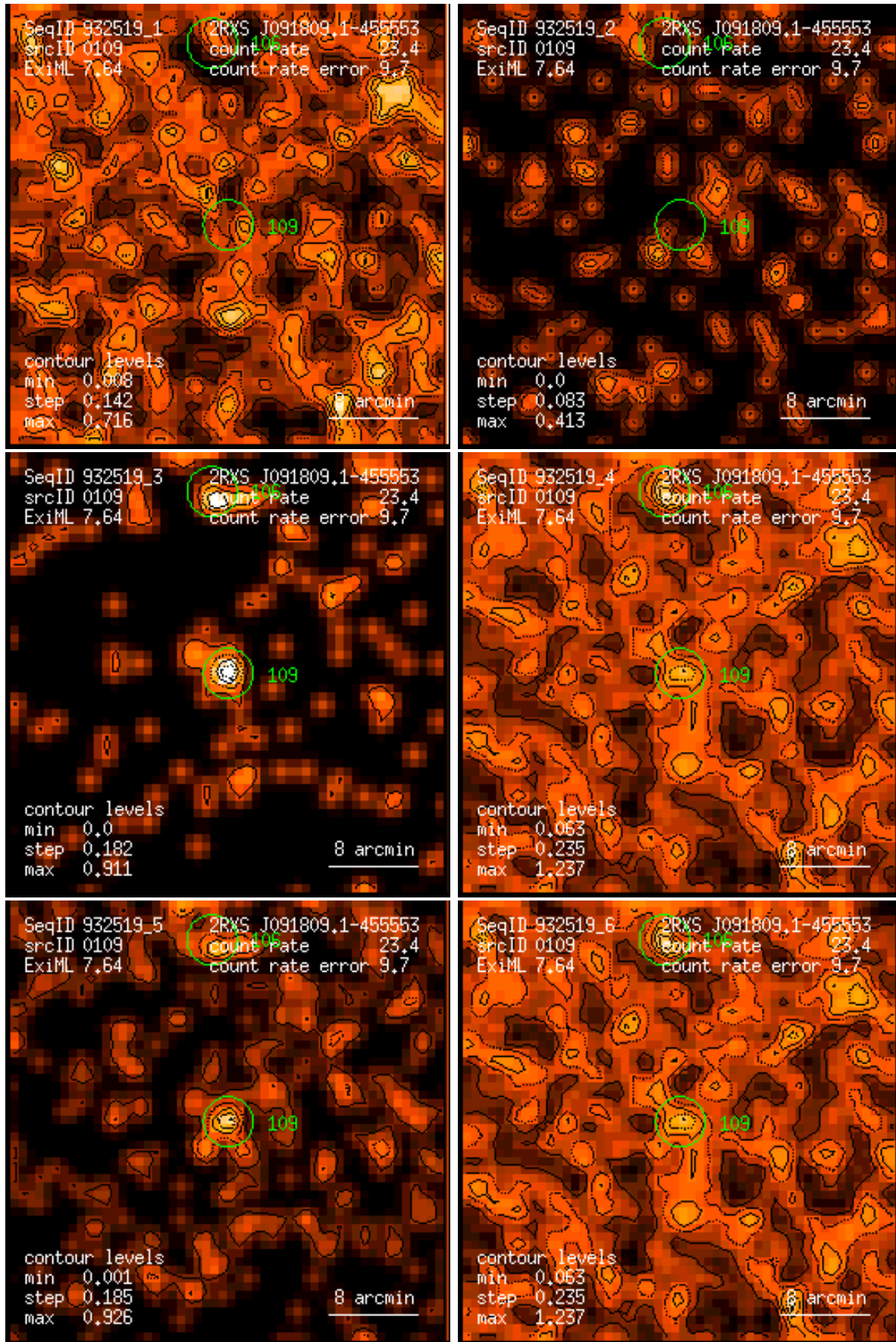
Figure 109: RASS 932519: detection 0109: band rate images, Gaussian filter: (1) PSPC channels 11 – 41, (2) 52 – 90, (3) 91 – 201, (4) 11 – 235, (5) 52 – 201, (6) 11 – 201. Broad band rates in counts/ks. Band rate contour levels in counts/ks/arcmin 2 .
