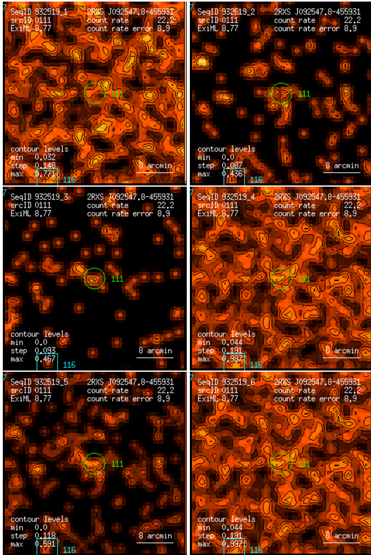
Figure 111: RASS 932519: detection 0111: band rate images, Gaussian filter: (1) PSPC channels 11 – 41, (2) 52 – 90, (3) 91 – 201, (4) 11 – 235, (5) 52 – 201, (6) 11 – 201. Broad band rates in counts/ks. Band rate contour levels in counts/ks/arcmin 2 .
