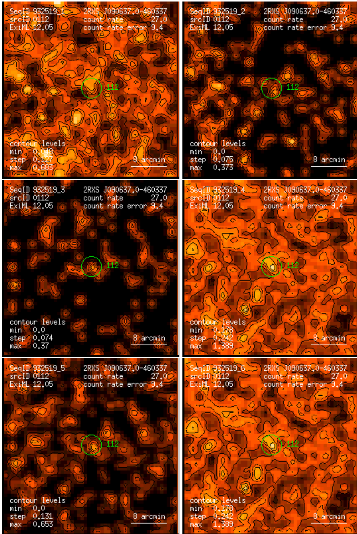
Figure 112: RASS 932519: detection 0112: band rate images, Gaussian filter: (1) PSPC channels 11 – 41, (2) 52 – 90, (3) 91 – 201, (4) 11 – 235, (5) 52 – 201, (6) 11 – 201. Broad band rates in counts/ks. Band rate contour levels in counts/ks/arcmin 2 .
