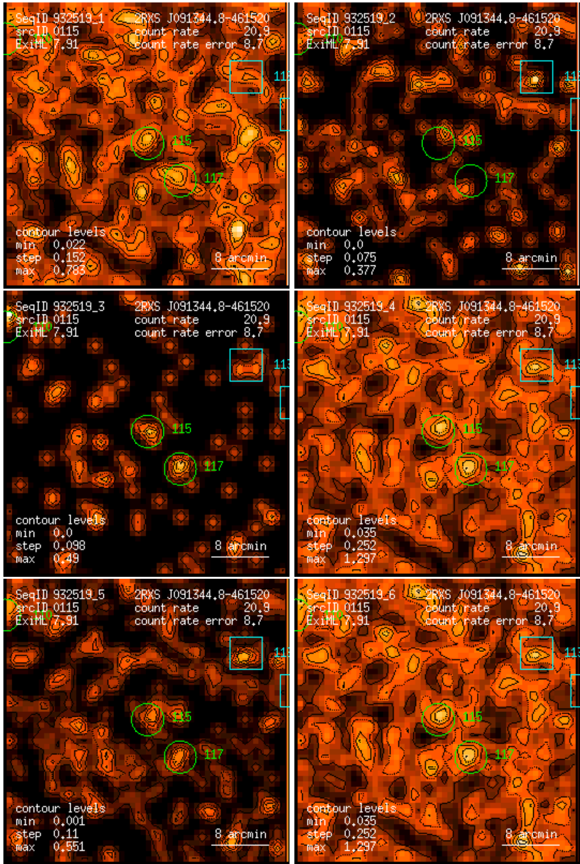
Figure 115: RASS 932519: detection 0115: band rate images, Gaussian filter: (1) PSPC channels 11 – 41, (2) 52 – 90, (3) 91 – 201, (4) 11 – 235, (5) 52 – 201, (6) 11 – 201. Broad band rates in counts/ks. Band rate contour levels in counts/ks/arcmin 2 .
