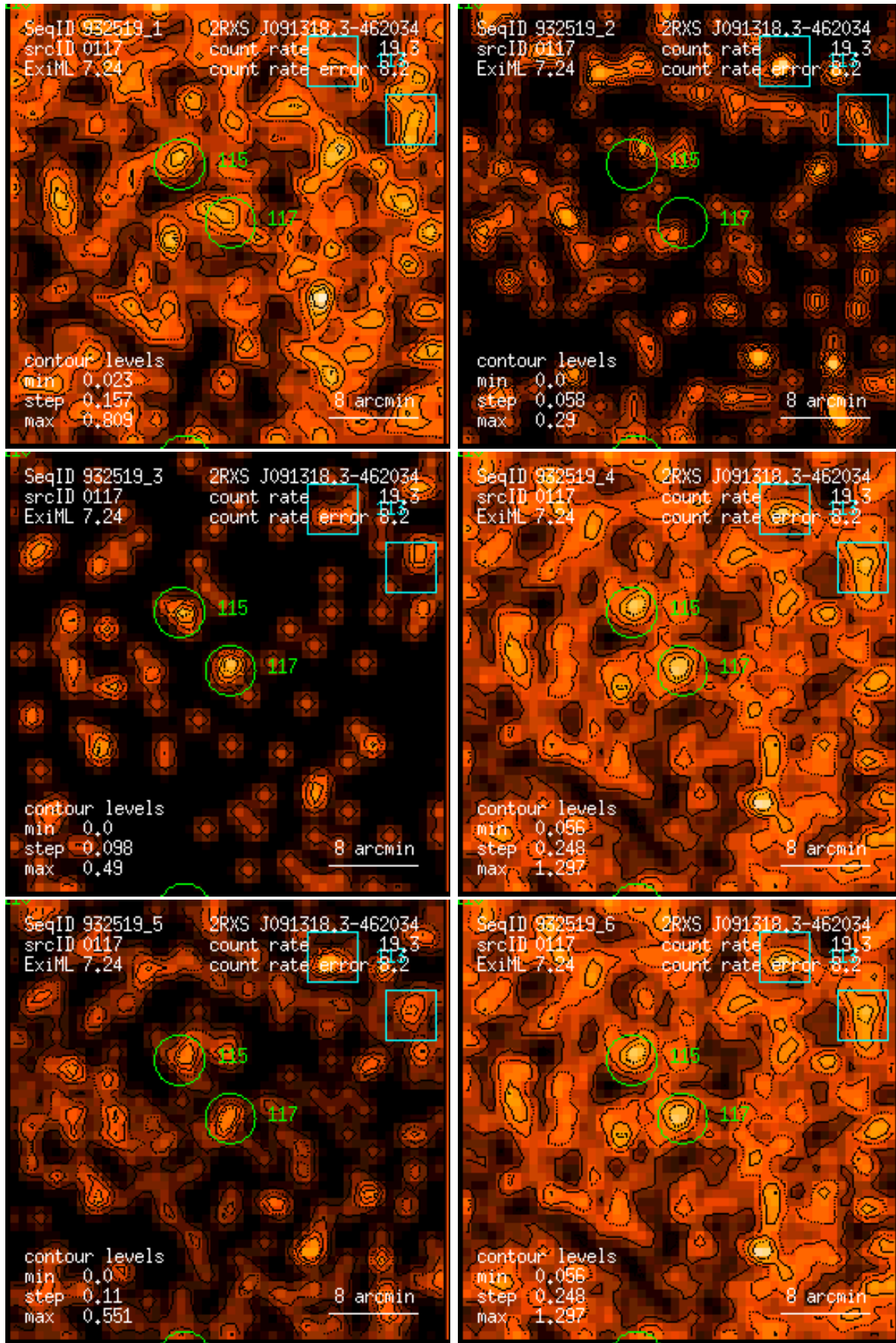
Figure 117: RASS 932519: detection 0117: band rate images, Gaussian filter: (1) PSPC channels 11 – 41, (2) 52 – 90, (3) 91 – 201, (4) 11 – 235, (5) 52 – 201, (6) 11 – 201. Broad band rates in counts/ks. Band rate contour levels in counts/ks/arcmin 2 .
