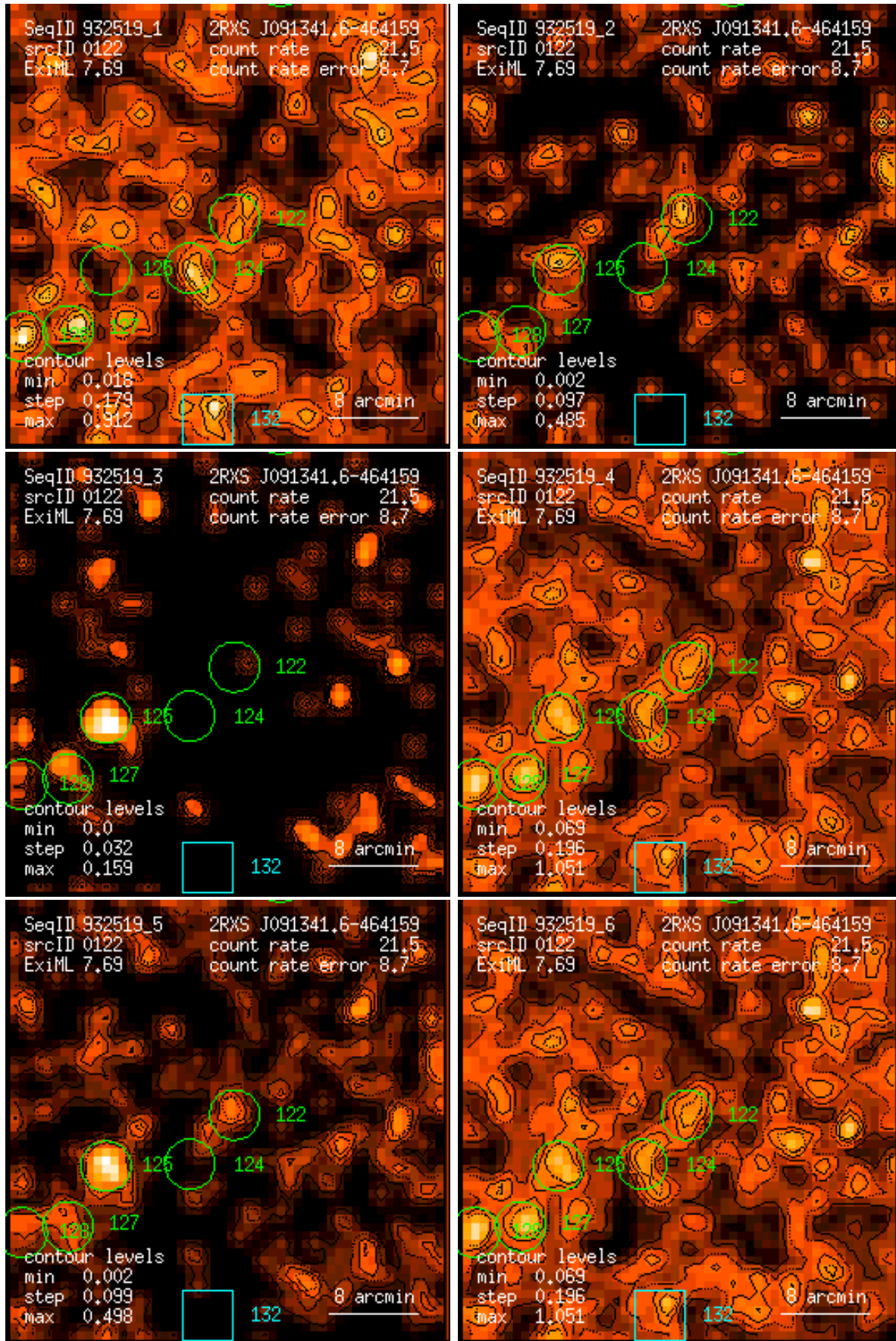
Figure 122: RASS 932519: detection 0122: band rate images, Gaussian filter: (1) PSPC channels 11 – 41, (2) 52 – 90, (3) 91 – 201, (4) 11 – 235, (5) 52 – 201, (6) 11 – 201. Broad band rates in counts/ks. Band rate contour levels in counts/ks/arcmin 2 .
