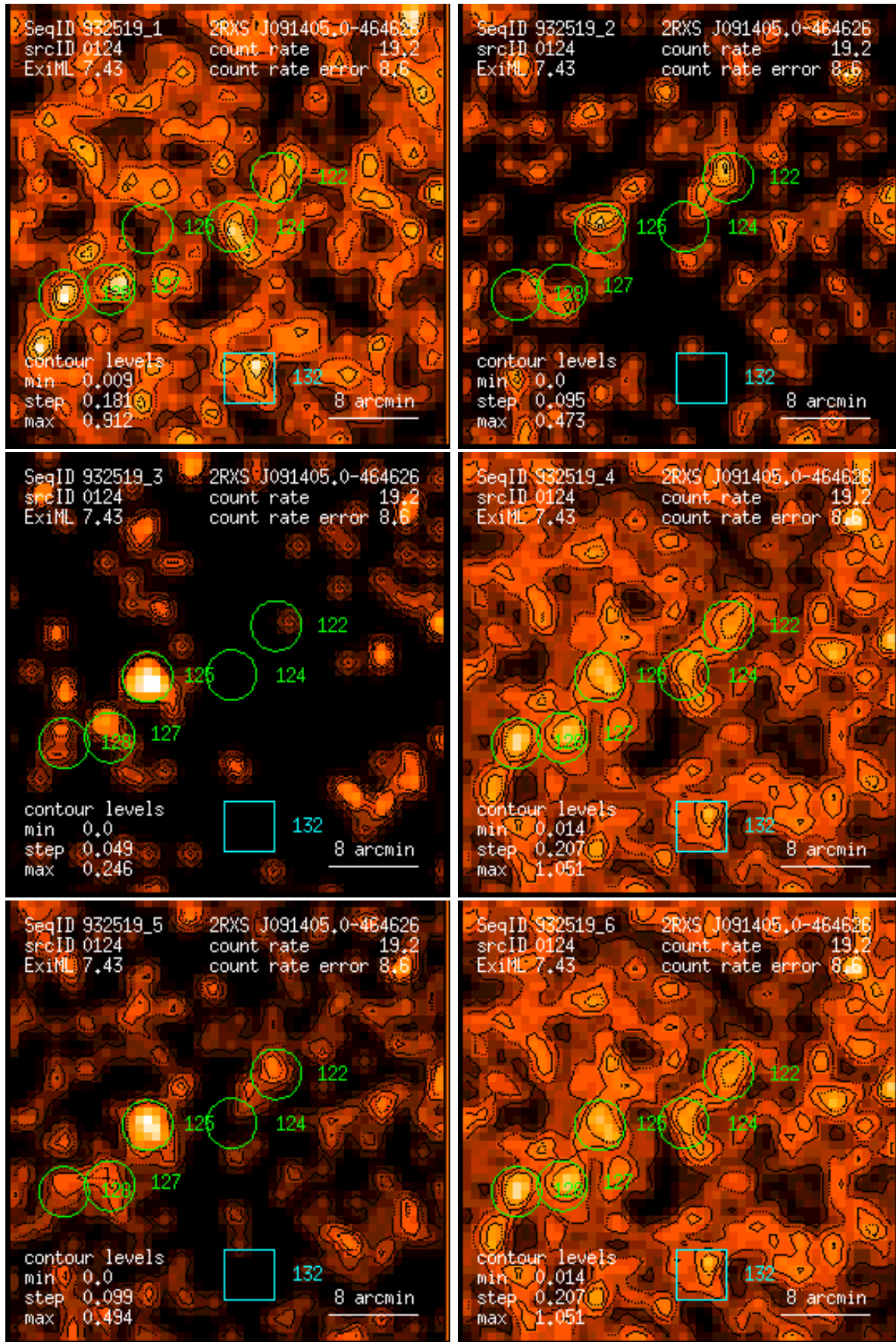
Figure 124: RASS 932519: detection 0124: band rate images, Gaussian filter: (1) PSPC channels 11 – 41, (2) 52 – 90, (3) 91 – 201, (4) 11 – 235, (5) 52 – 201, (6) 11 – 201. Broad band rates in counts/ks. Band rate contour levels in counts/ks/arcmin 2 .
