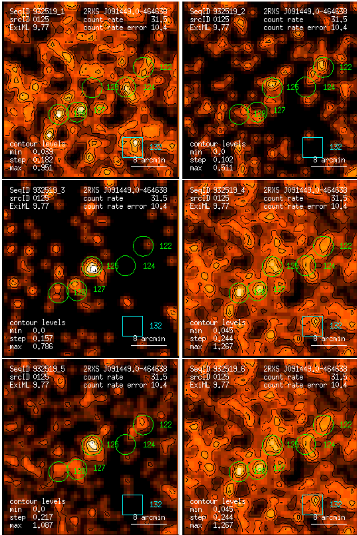
Figure 125: RASS 932519: detection 0125: band rate images, Gaussian filter: (1) PSPC channels 11 – 41, (2) 52 – 90, (3) 91 – 201, (4) 11 – 235, (5) 52 – 201, (6) 11 – 201. Broad band rates in counts/ks. Band rate contour levels in counts/ks/arcmin 2 .
