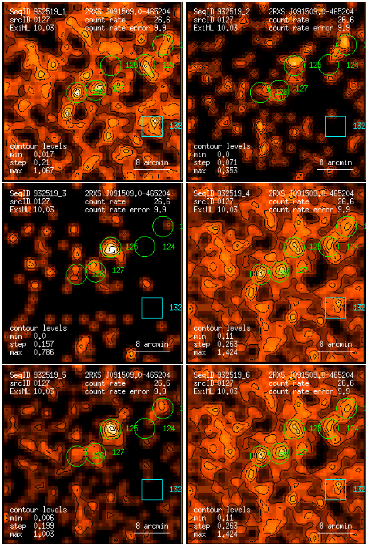
Figure 127: RASS 932519: detection 0127: band rate images, Gaussian filter: (1) PSPC channels 11 – 41, (2) 52 – 90, (3) 91 – 201, (4) 11 – 235, (5) 52 – 201, (6) 11 – 201. Broad band rates in counts/ks. Band rate contour levels in counts/ks/arcmin 2 .
