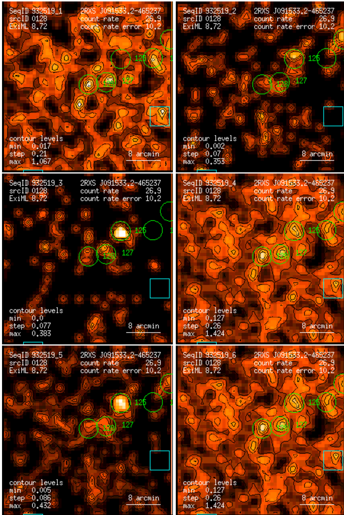
Figure 128: RASS 932519: detection 0128: band rate images, Gaussian filter: (1) PSPC channels 11 – 41, (2) 52 – 90, (3) 91 – 201, (4) 11 – 235, (5) 52 – 201, (6) 11 – 201. Broad band rates in counts/ks. Band rate contour levels in counts/ks/arcmin 2 .
