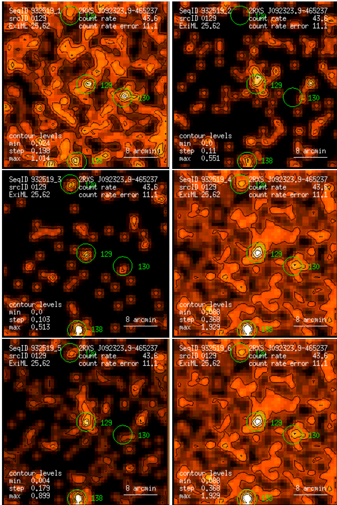
Figure 129: RASS 932519: detection 0129: band rate images, Gaussian filter: (1) PSPC channels 11 – 41, (2) 52 – 90, (3) 91 – 201, (4) 11 – 235, (5) 52 – 201, (6) 11 – 201. Broad band rates in counts/ks. Band rate contour levels in counts/ks/arcmin 2 .
