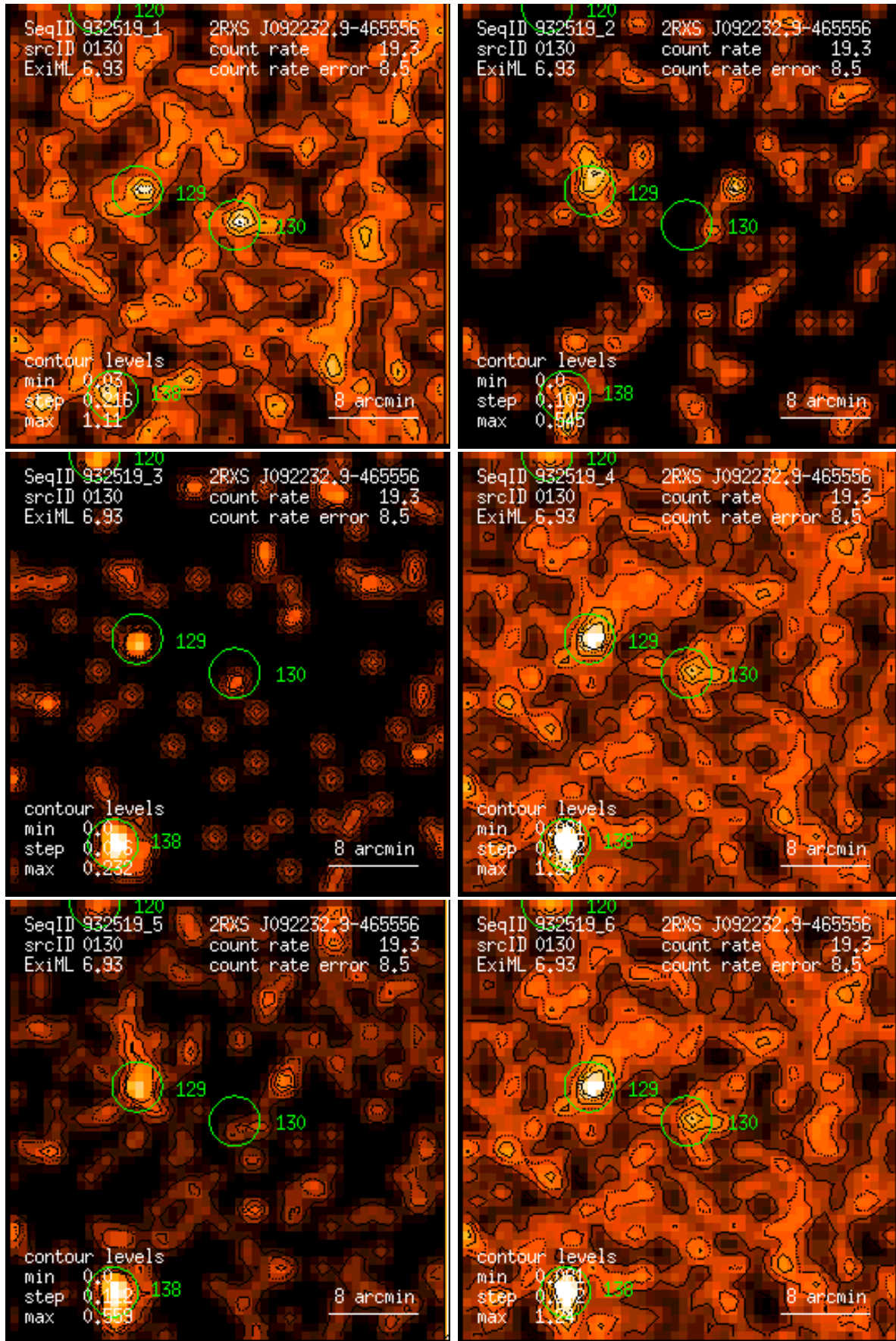
Figure 130: RASS 932519: detection 0130: band rate images, Gaussian filter: (1) PSPC channels 11 – 41, (2) 52 – 90, (3) 91 – 201, (4) 11 – 235, (5) 52 – 201, (6) 11 – 201. Broad band rates in counts/ks. Band rate contour levels in counts/ks/arcmin 2 .
