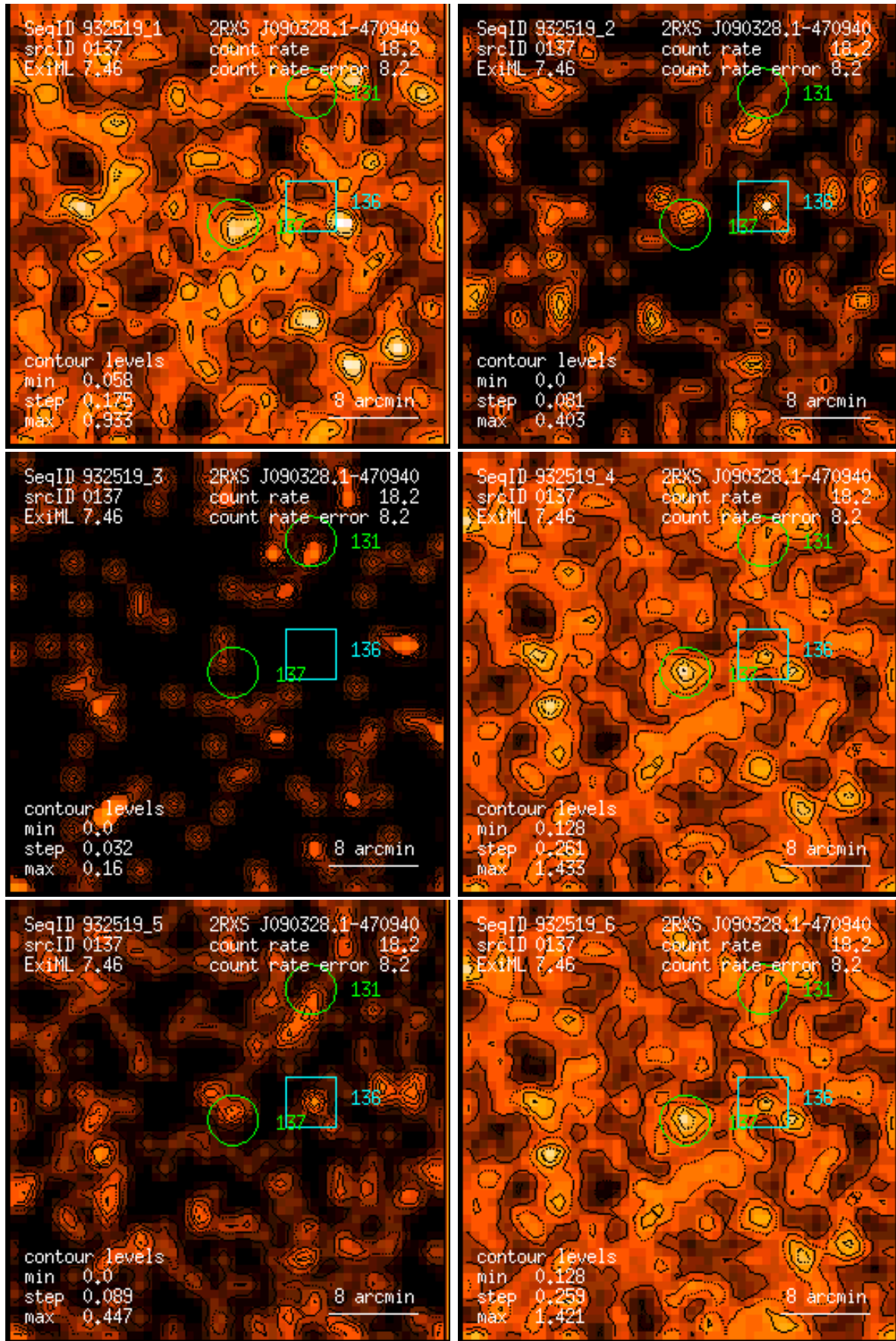
Figure 137: RASS 932519: detection 0137: band rate images, Gaussian filter: (1) PSPC channels 11 – 41, (2) 52 – 90, (3) 91 – 201, (4) 11 – 235, (5) 52 – 201, (6) 11 – 201. Broad band rates in counts/ks. Band rate contour levels in counts/ks/arcmin 2 .
