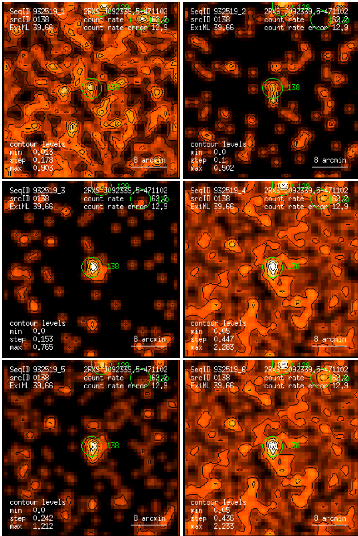
Figure 138: RASS 932519: detection 0138: band rate images, Gaussian filter: (1) PSPC channels 11 – 41, (2) 52 – 90, (3) 91 – 201, (4) 11 – 235, (5) 52 – 201, (6) 11 – 201. Broad band rates in counts/ks. Band rate contour levels in counts/ks/arcmin 2 .
