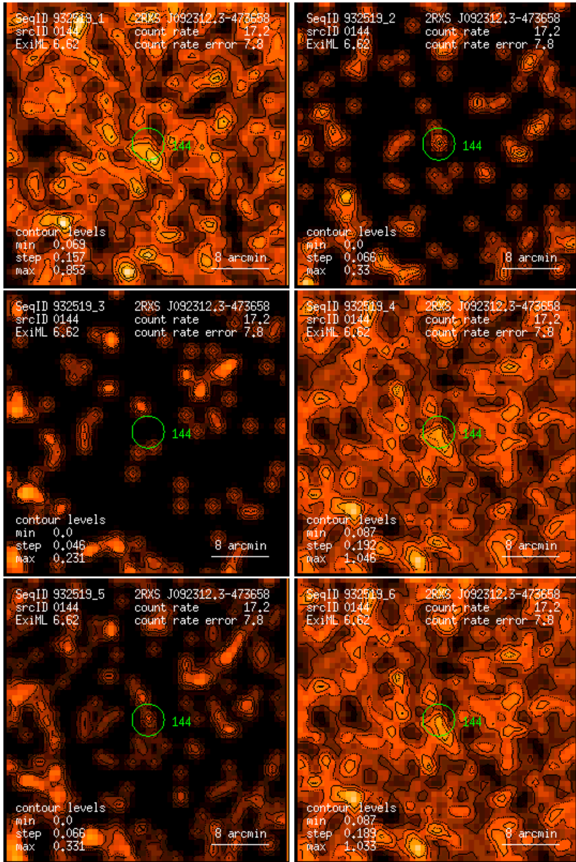
Figure 144: RASS 932519: detection 0144: band rate images, Gaussian filter: (1) PSPC channels 11 – 41, (2) 52 – 90, (3) 91 – 201, (4) 11 – 235, (5) 52 – 201, (6) 11 – 201. Broad band rates in counts/ks. Band rate contour levels in counts/ks/arcmin 2 .
