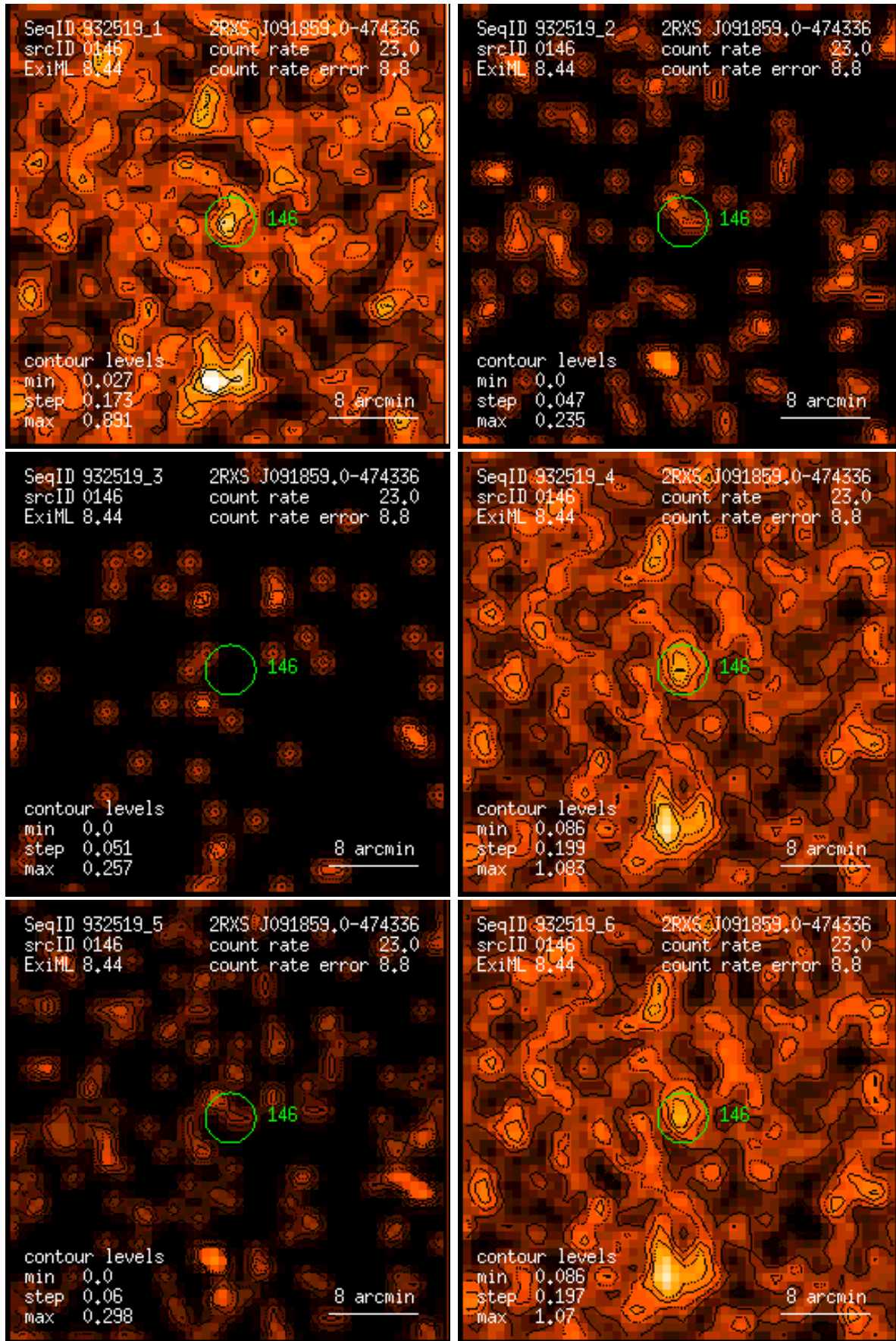
Figure 146: RASS 932519: detection 0146: band rate images, Gaussian filter: (1) PSPC channels 11 – 41, (2) 52 – 90, (3) 91 – 201, (4) 11 – 235, (5) 52 – 201, (6) 11 – 201. Broad band rates in counts/ks. Band rate contour levels in counts/ks/arcmin 2 .
