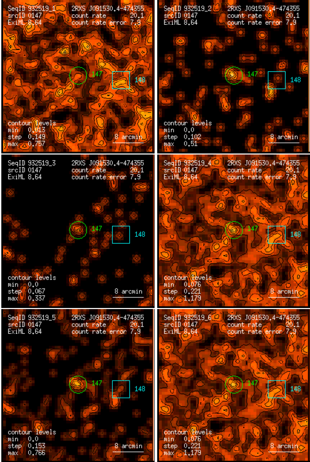
Figure 147: RASS 932519: detection 0147: band rate images, Gaussian filter: (1) PSPC channels 11 – 41, (2) 52 – 90, (3) 91 – 201, (4) 11 – 235, (5) 52 – 201, (6) 11 – 201. Broad band rates in counts/ks. Band rate contour levels in counts/ks/arcmin 2 .
