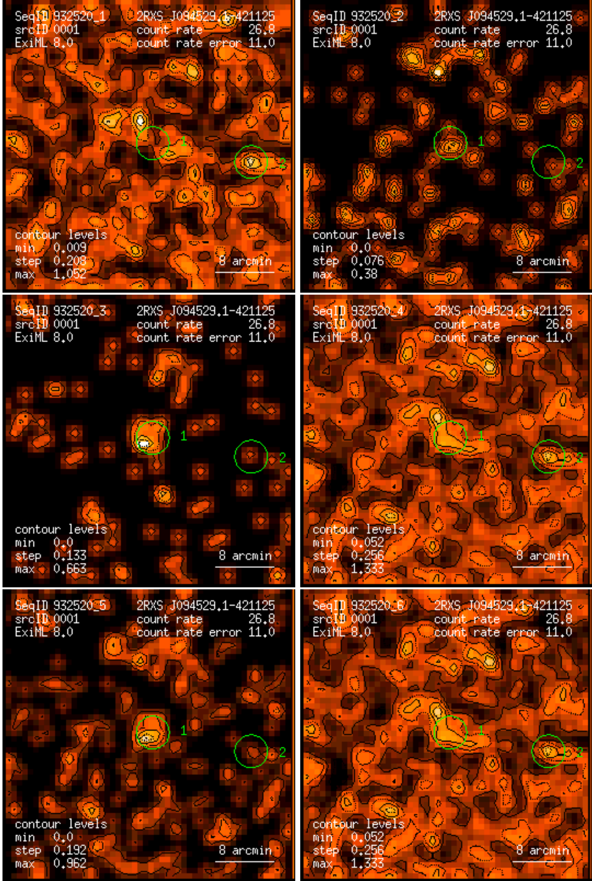
Figure 1: RASS 932520: detection 0001: band rate images, Gaussian filter: (1) PSPC channels 11 – 41, (2) 52 – 90, (3) 91 – 201, (4) 11 – 235, (5) 52 – 201, (6) 11 – 201. Broad band rates in counts/ks. Band rate contour levels in counts/ks/arcmin 2 .
