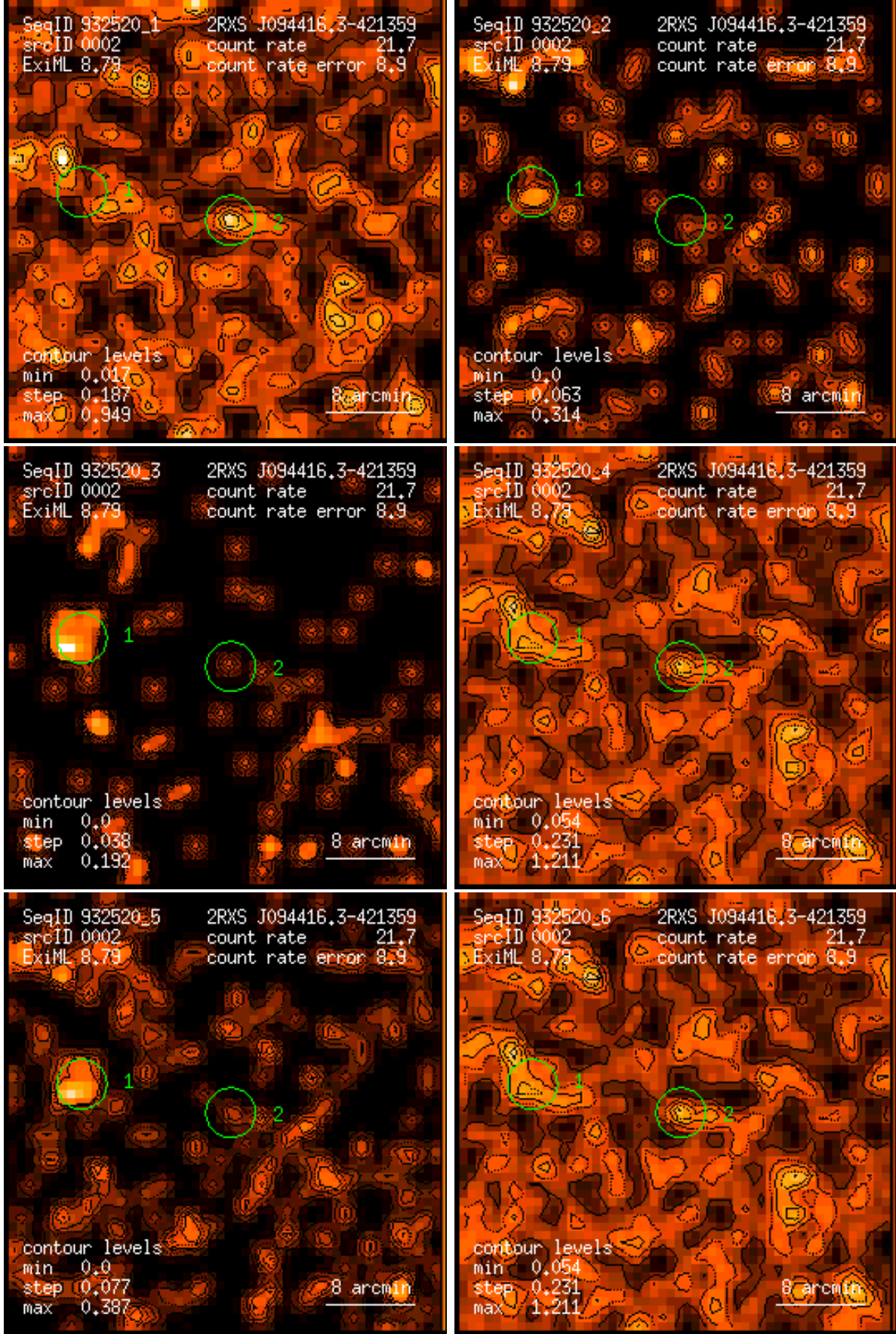
Figure 2: RASS 932520: detection 0002: band rate images, Gaussian filter: (1) PSPC channels 11 – 41, (2) 52 – 90, (3) 91 – 201, (4) 11 – 235, (5) 52 – 201, (6) 11 – 201. Broad band rates in counts/ks. Band rate contour levels in counts/ks/arcmin 2 .
