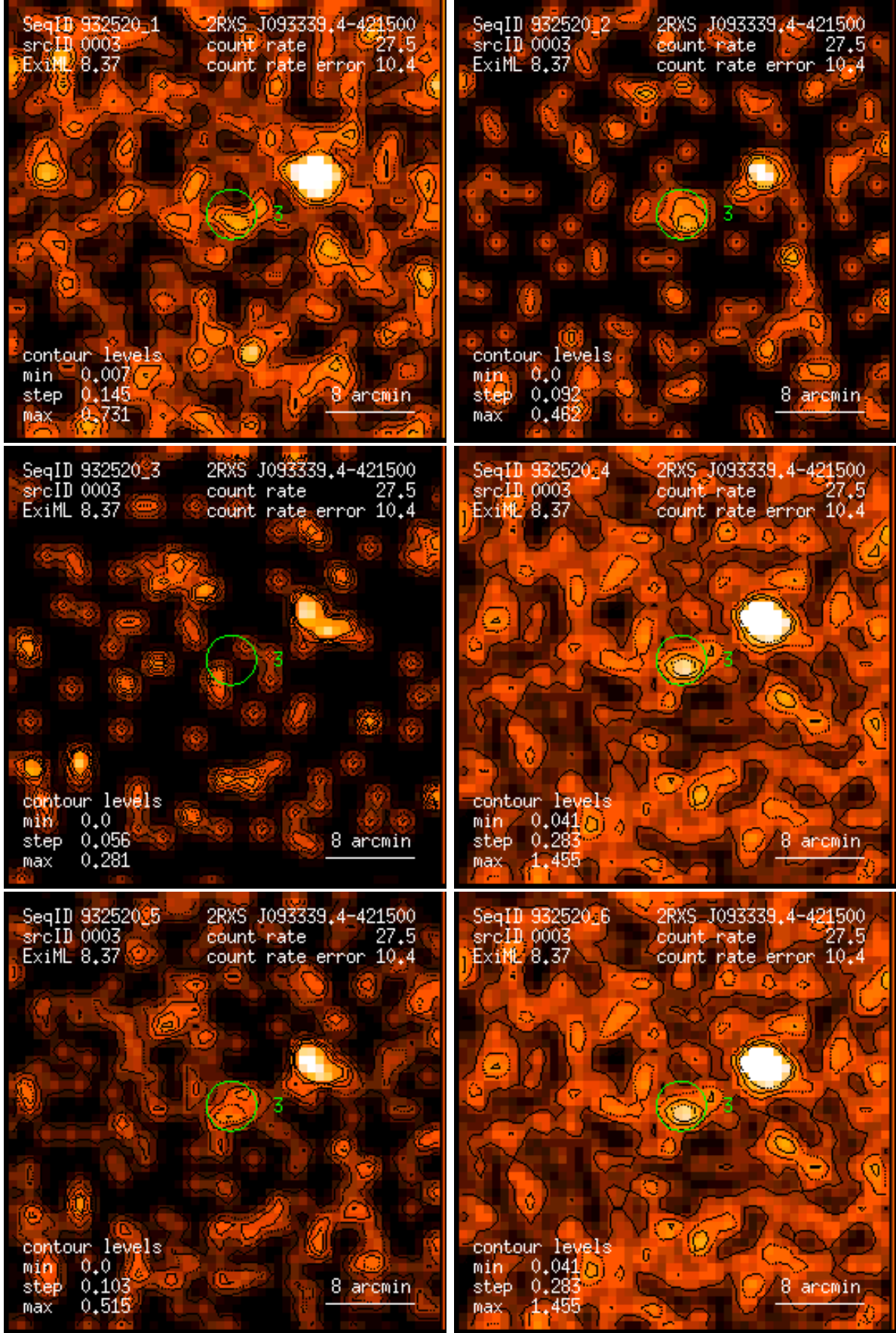
Figure 3: RASS 932520: detection 0003: band rate images, Gaussian filter: (1) PSPC channels 11 – 41, (2) 52 – 90, (3) 91 – 201, (4) 11 – 235, (5) 52 – 201, (6) 11 – 201. Broad band rates in counts/ks. Band rate contour levels in counts/ks/arcmin 2 .
