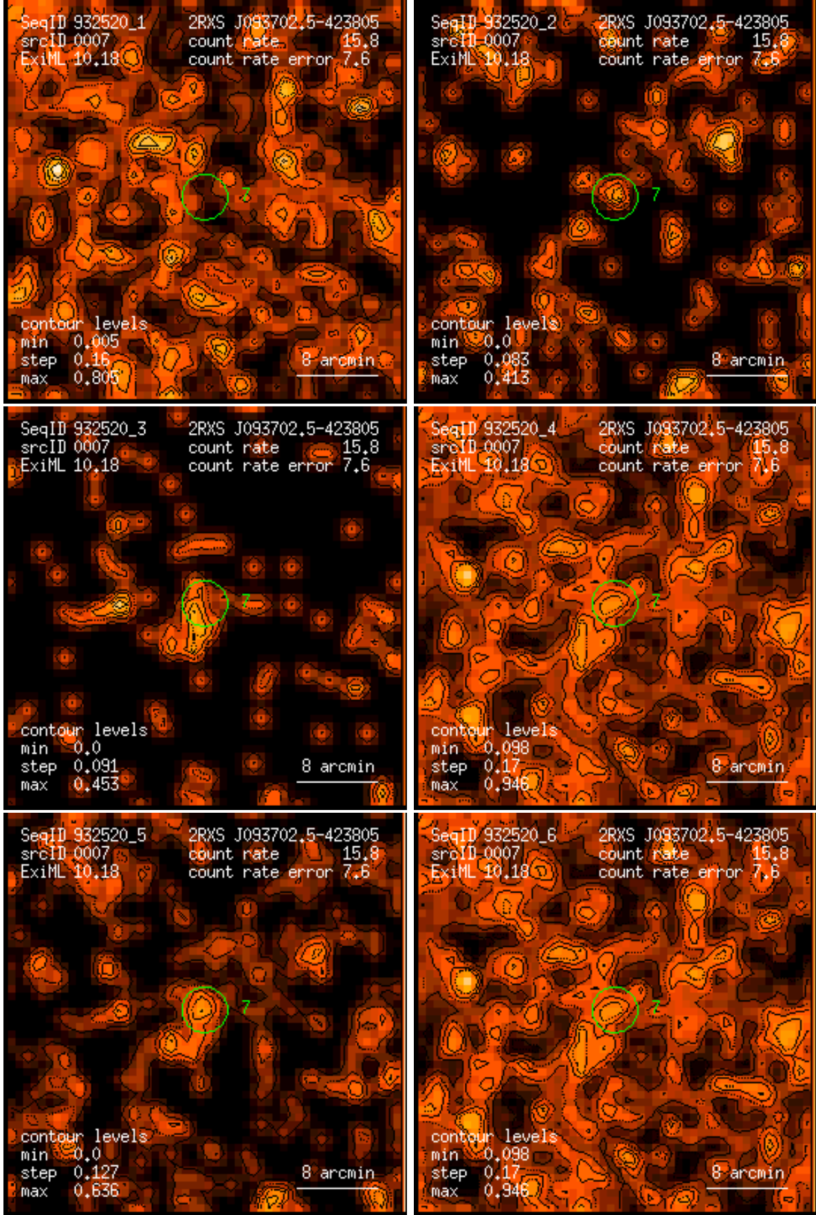
Figure 7: RASS 932520: detection 0007: band rate images, Gaussian filter: (1) PSPC channels 11 – 41, (2) 52 – 90, (3) 91 – 201, (4) 11 – 235, (5) 52 – 201, (6) 11 – 201. Broad band rates in counts/ks. Band rate contour levels in counts/ks/arcmin 2 .
