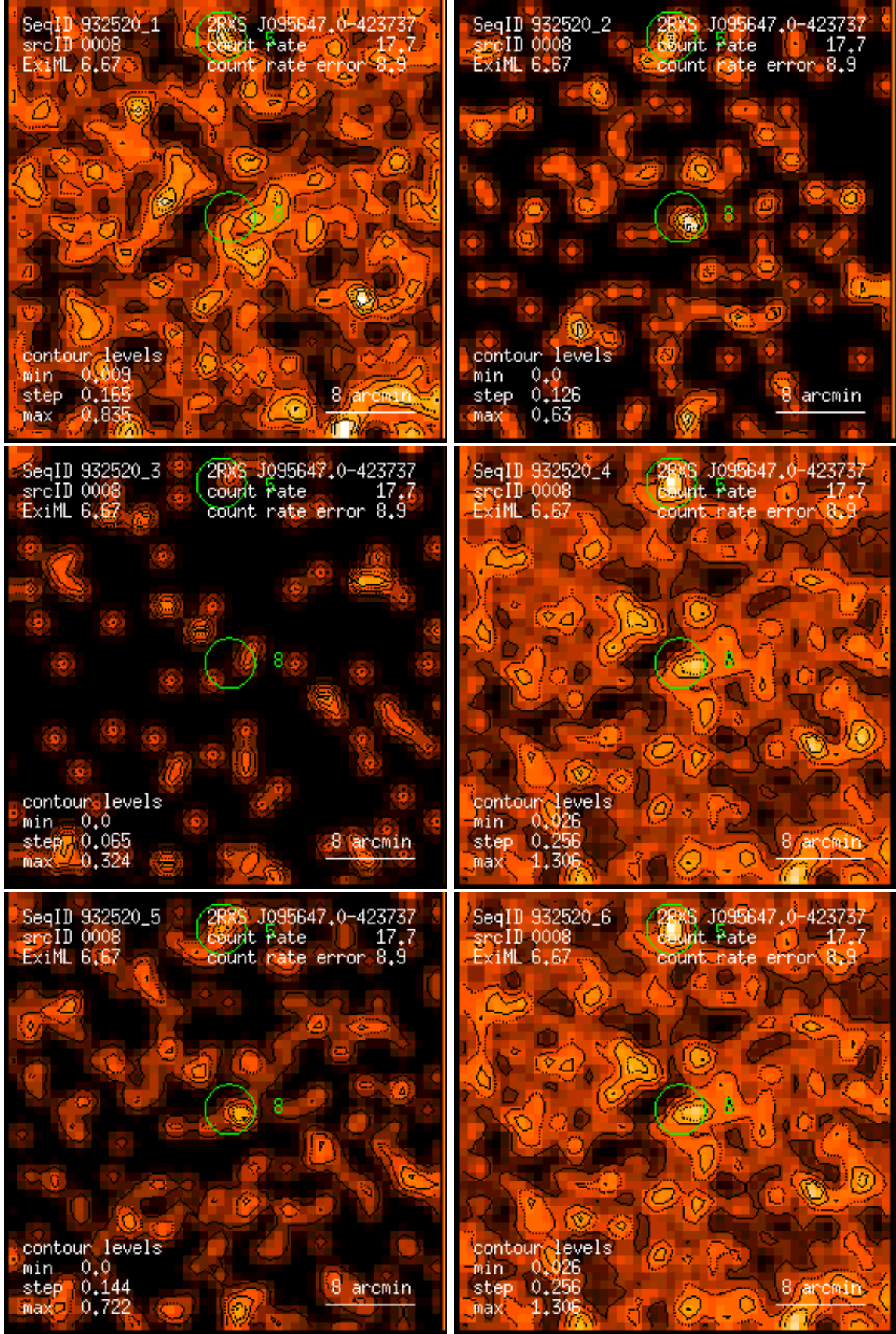
Figure 8: RASS 932520: detection 0008: band rate images, Gaussian filter: (1) PSPC channels 11 – 41, (2) 52 – 90, (3) 91 – 201, (4) 11 – 235, (5) 52 – 201, (6) 11 – 201. Broad band rates in counts/ks. Band rate contour levels in counts/ks/arcmin 2 .
