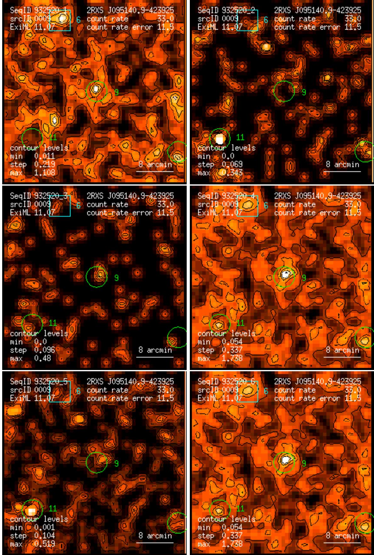
Figure 9: RASS 932520: detection 0009: band rate images, Gaussian filter: (1) PSPC channels 11 – 41, (2) 52 – 90, (3) 91 – 201, (4) 11 – 235, (5) 52 – 201, (6) 11 – 201. Broad band rates in counts/ks. Band rate contour levels in counts/ks/arcmin 2 .
