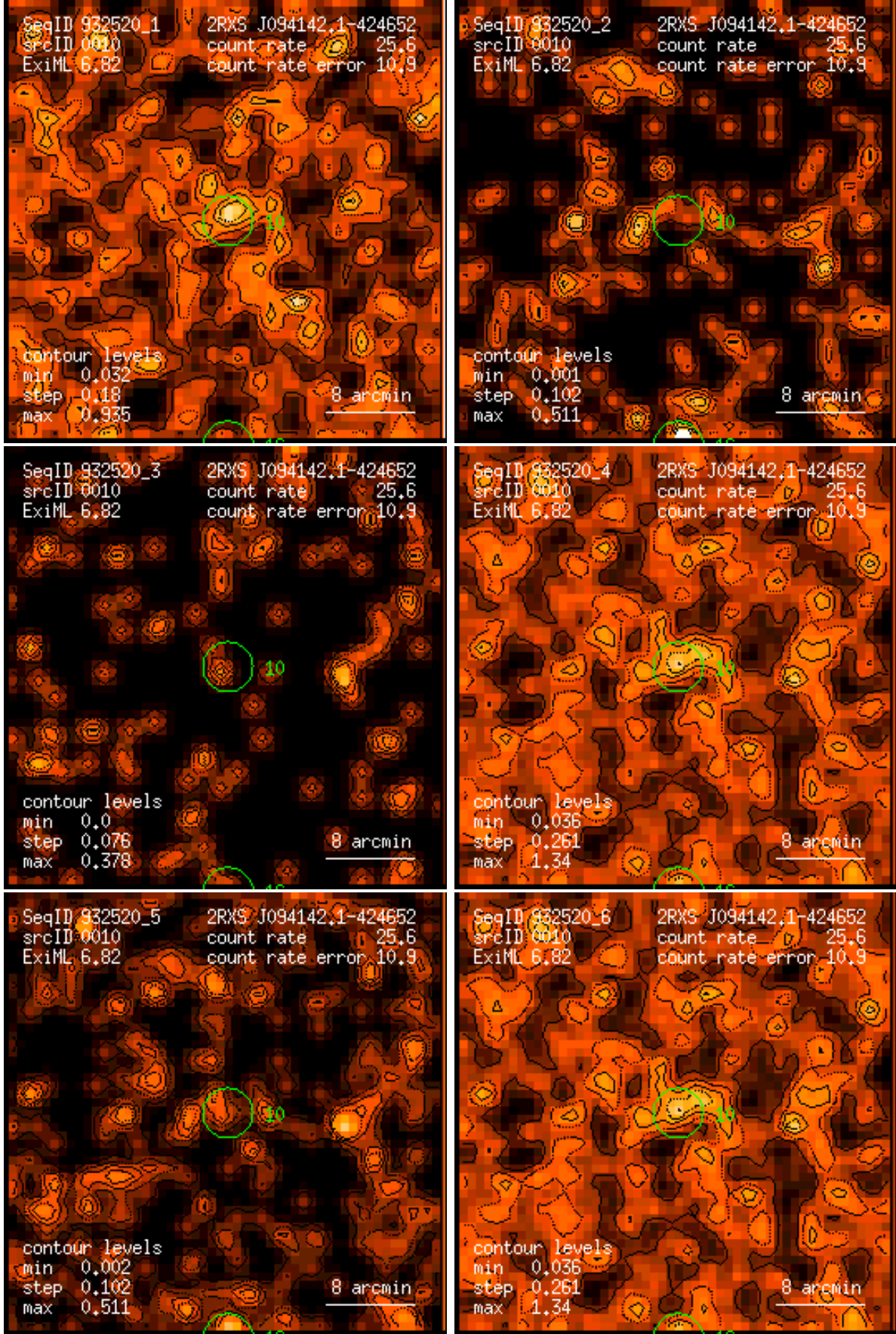
Figure 10: RASS 932520: detection 0010: band rate images, Gaussian filter: (1) PSPC channels 11 – 41, (2) 52 – 90, (3) 91 – 201, (4) 11 – 235, (5) 52 – 201, (6) 11 – 201. Broad band rates in counts/ks. Band rate contour levels in counts/ks/arcmin 2 .
