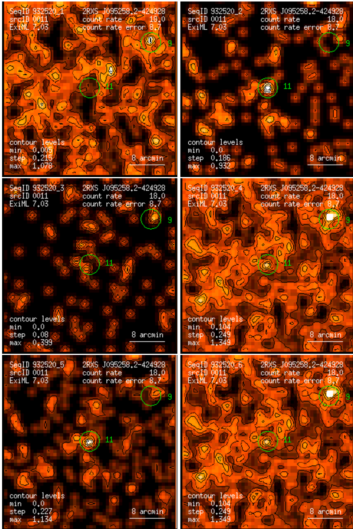
Figure 11: RASS 932520: detection 0011: band rate images, Gaussian filter: (1) PSPC channels 11 – 41, (2) 52 – 90, (3) 91 – 201, (4) 11 – 235, (5) 52 – 201, (6) 11 – 201. Broad band rates in counts/ks. Band rate contour levels in counts/ks/arcmin 2 .
