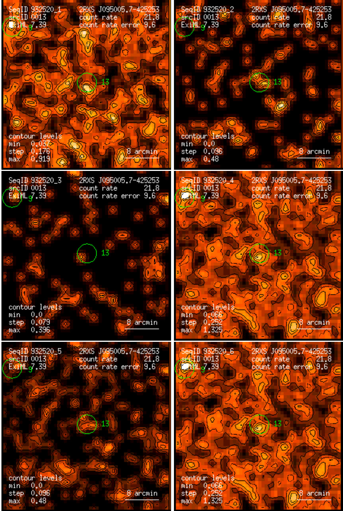
Figure 13: RASS 932520: detection 0013: band rate images, Gaussian filter: (1) PSPC channels 11 – 41, (2) 52 – 90, (3) 91 – 201, (4) 11 – 235, (5) 52 – 201, (6) 11 – 201. Broad band rates in counts/ks. Band rate contour levels in counts/ks/arcmin 2 .
