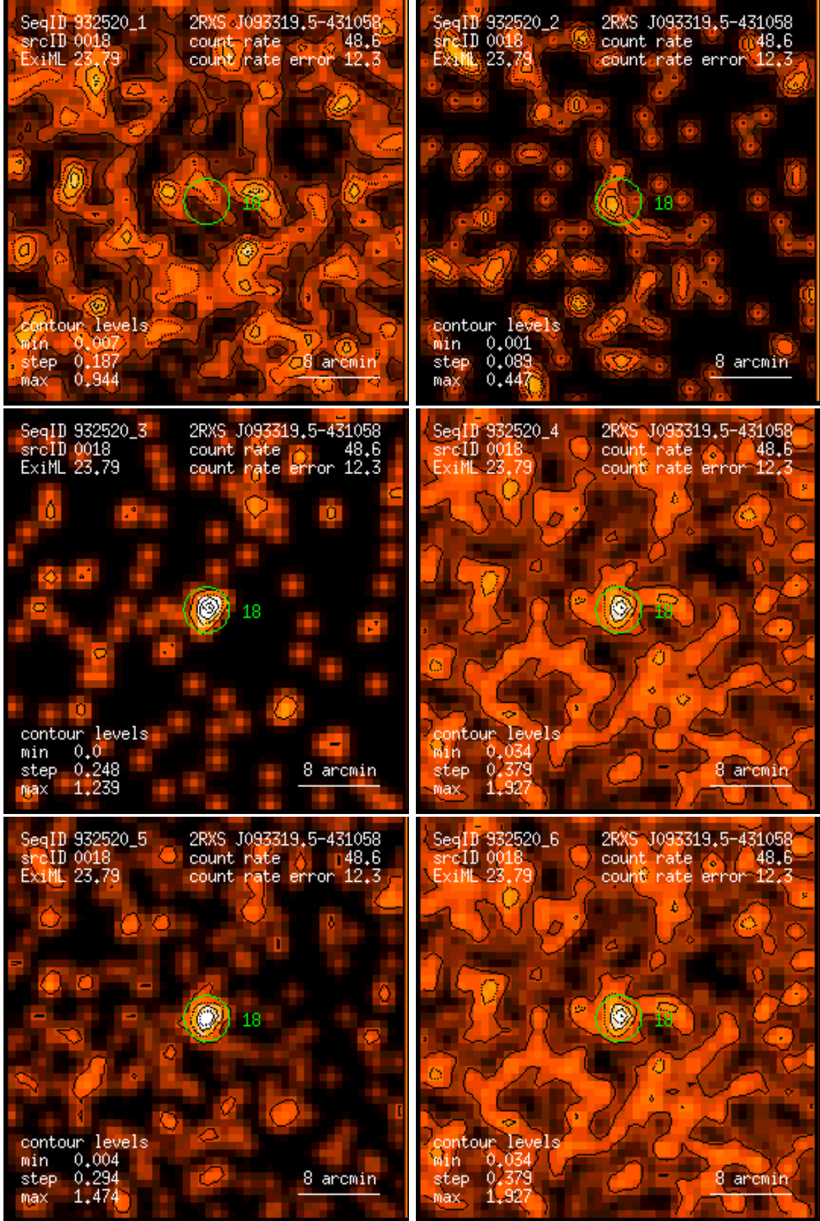
Figure 18: RASS 932520: detection 0018: band rate images, Gaussian filter: (1) PSPC channels 11 – 41, (2) 52 – 90, (3) 91 – 201, (4) 11 – 235, (5) 52 – 201, (6) 11 – 201. Broad band rates in counts/ks. Band rate contour levels in counts/ks/arcmin 2 .
