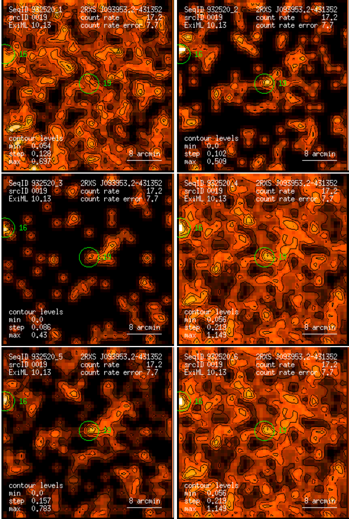
Figure 19: RASS 932520: detection 0019: band rate images, Gaussian filter: (1) PSPC channels 11 – 41, (2) 52 – 90, (3) 91 – 201, (4) 11 – 235, (5) 52 – 201, (6) 11 – 201. Broad band rates in counts/ks. Band rate contour levels in counts/ks/arcmin 2 .
