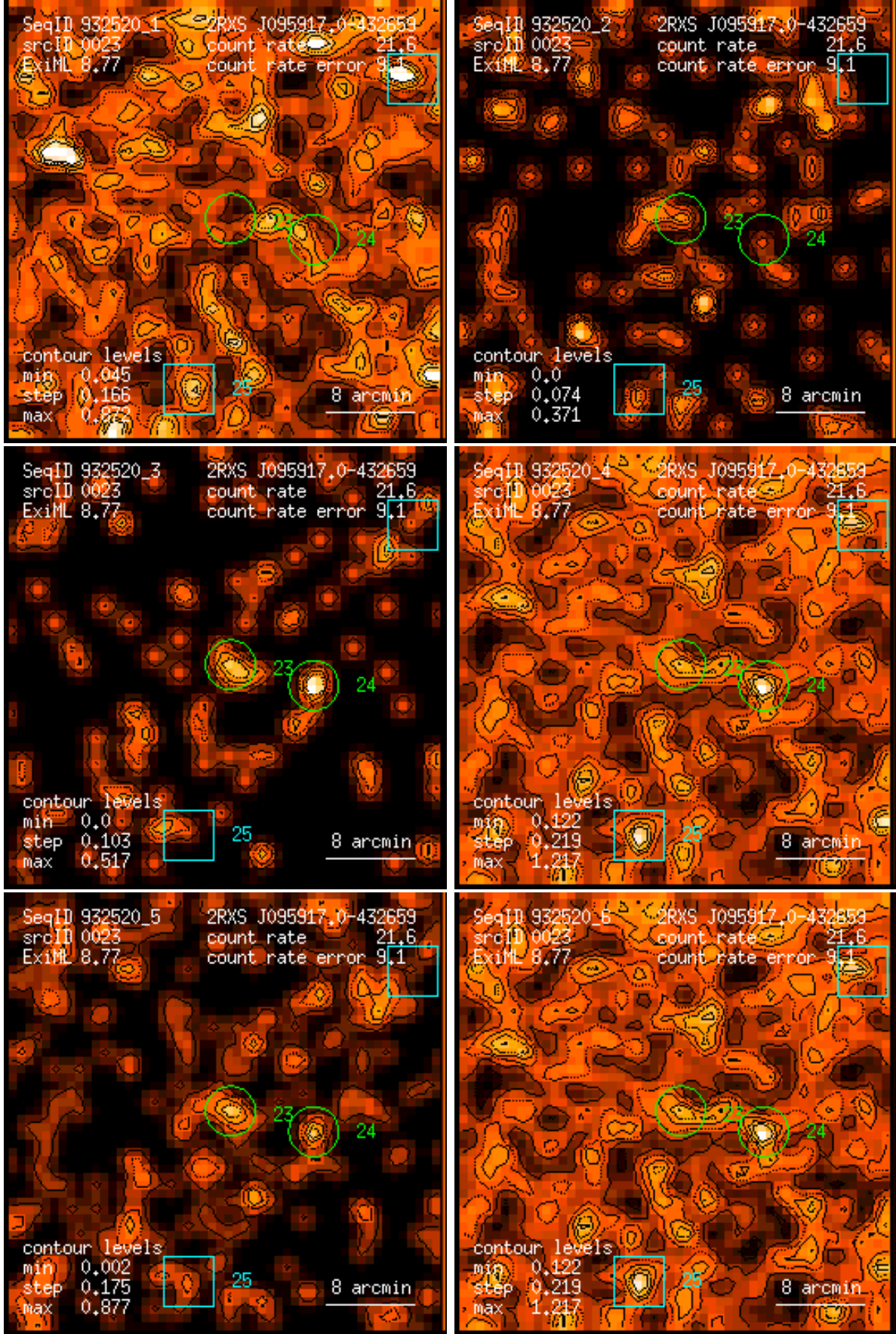
Figure 23: RASS 932520: detection 0023: band rate images, Gaussian filter: (1) PSPC channels 11 – 41, (2) 52 – 90, (3) 91 – 201, (4) 11 – 235, (5) 52 – 201, (6) 11 – 201. Broad band rates in counts/ks. Band rate contour levels in counts/ks/arcmin 2 .
