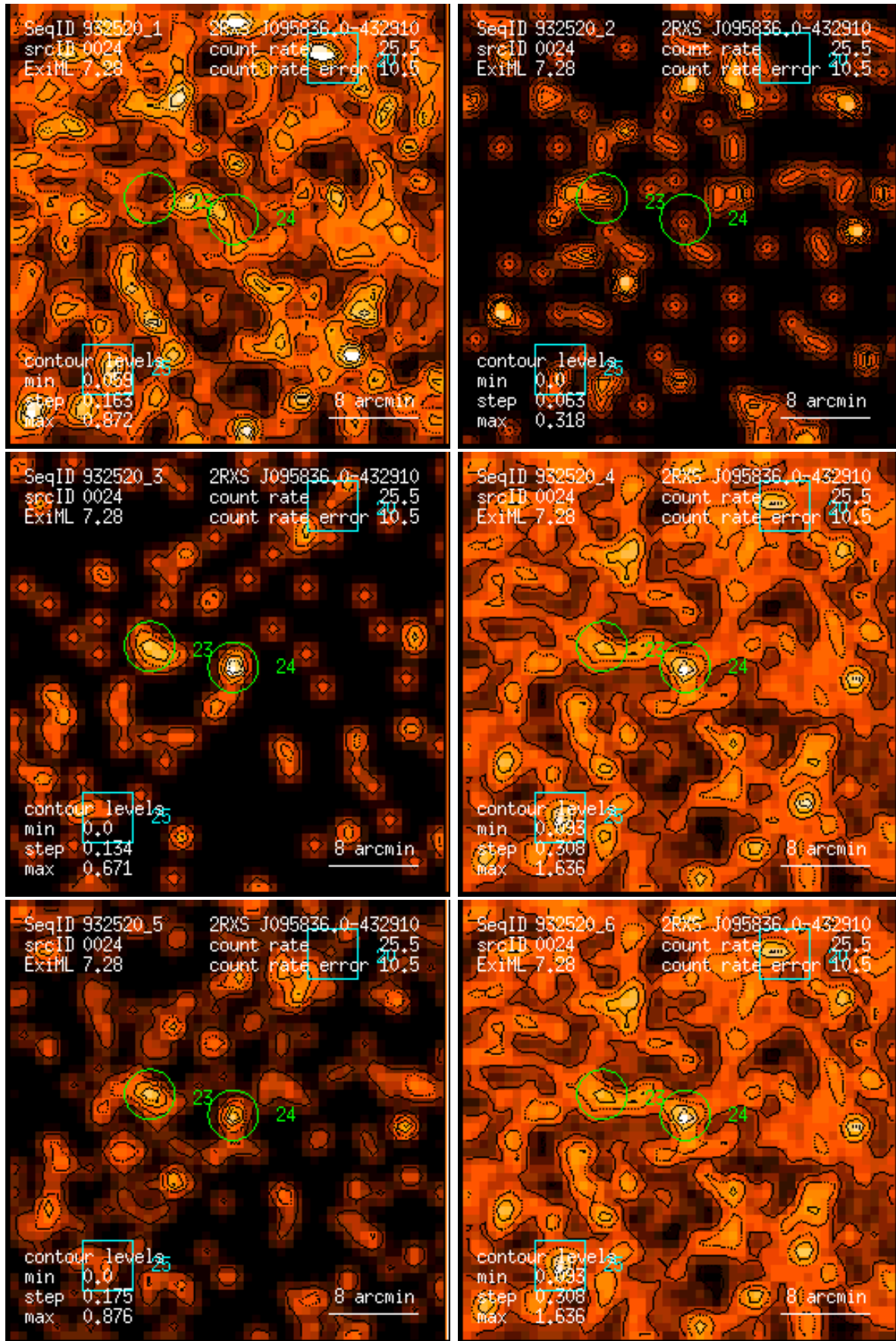
Figure 24: RASS 932520: detection 0024: band rate images, Gaussian filter: (1) PSPC channels 11 – 41, (2) 52 – 90, (3) 91 – 201, (4) 11 – 235, (5) 52 – 201, (6) 11 – 201. Broad band rates in counts/ks. Band rate contour levels in counts/ks/arcmin 2 .
