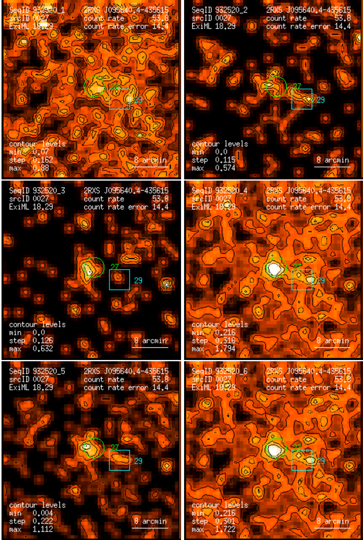
Figure 27: RASS 932520: detection 0027: band rate images, Gaussian filter: (1) PSPC channels 11 – 41, (2) 52 – 90, (3) 91 – 201, (4) 11 – 235, (5) 52 – 201, (6) 11 – 201. Broad band rates in counts/ks. Band rate contour levels in counts/ks/arcmin 2 .
