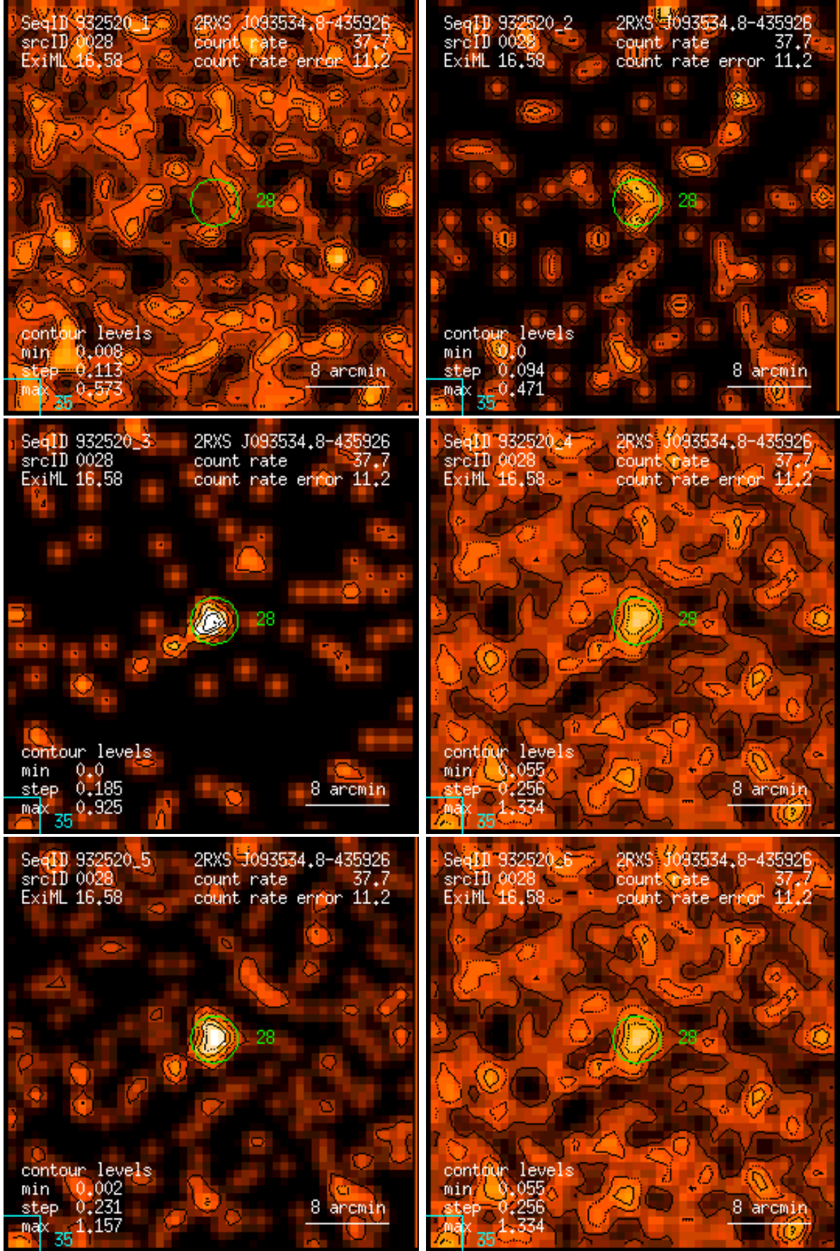
Figure 28: RASS 932520: detection 0028: band rate images, Gaussian filter: (1) PSPC channels 11 – 41, (2) 52 – 90, (3) 91 – 201, (4) 11 – 235, (5) 52 – 201, (6) 11 – 201. Broad band rates in counts/ks. Band rate contour levels in counts/ks/arcmin 2 .
