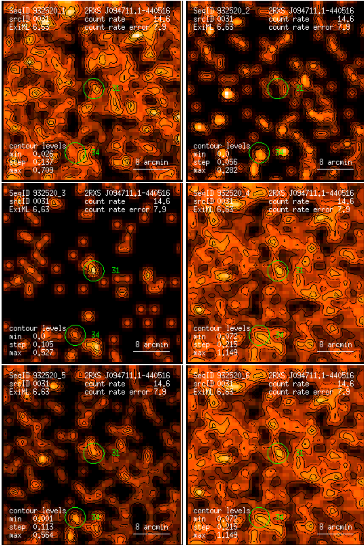
Figure 31: RASS 932520: detection 0031: band rate images, Gaussian filter: (1) PSPC channels 11 – 41, (2) 52 – 90, (3) 91 – 201, (4) 11 – 235, (5) 52 – 201, (6) 11 – 201. Broad band rates in counts/ks. Band rate contour levels in counts/ks/arcmin 2 .
