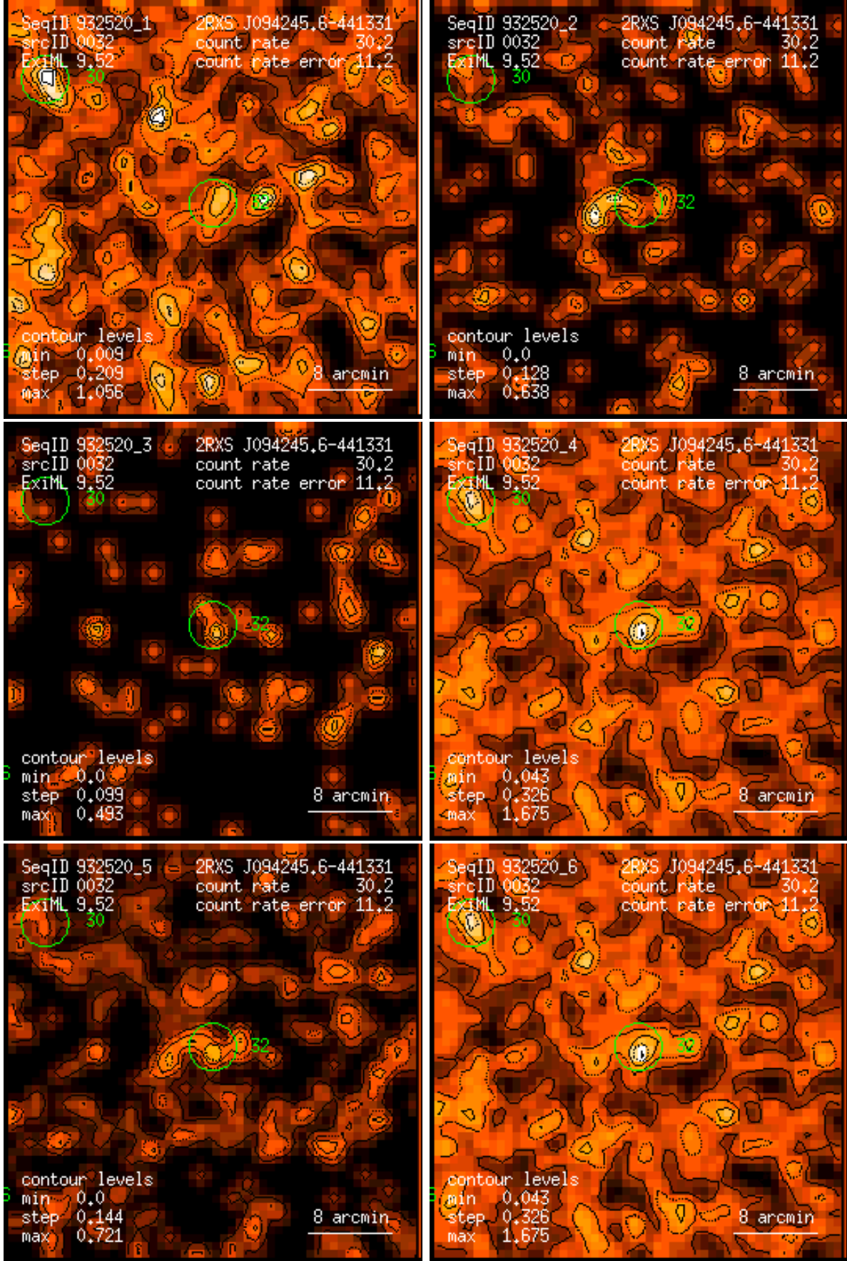
Figure 32: RASS 932520: detection 0032: band rate images, Gaussian filter: (1) PSPC channels 11 – 41, (2) 52 – 90, (3) 91 – 201, (4) 11 – 235, (5) 52 – 201, (6) 11 – 201. Broad band rates in counts/ks. Band rate contour levels in counts/ks/arcmin 2 .
