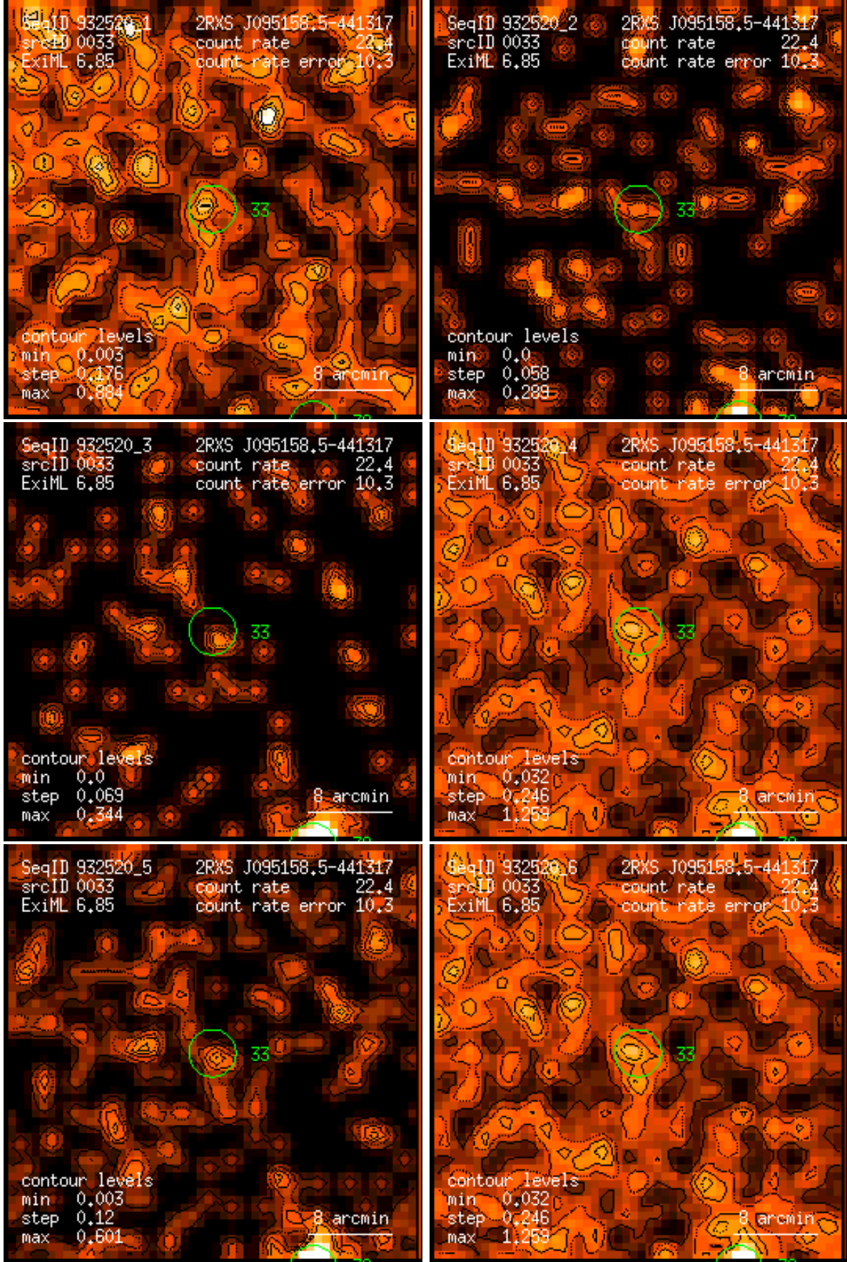
Figure 33: RASS 932520: detection 0033: band rate images, Gaussian filter: (1) PSPC channels 11 – 41, (2) 52 – 90, (3) 91 – 201, (4) 11 – 235, (5) 52 – 201, (6) 11 – 201. Broad band rates in counts/ks. Band rate contour levels in counts/ks/arcmin 2 .
