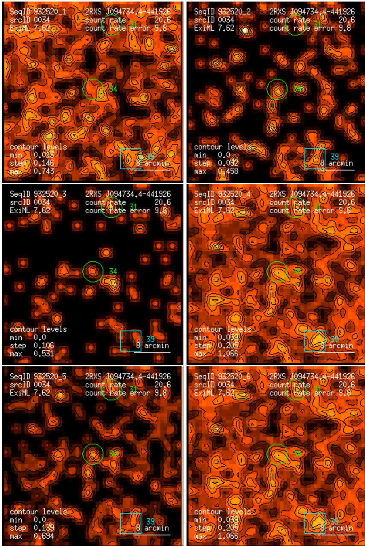
Figure 34: RASS 932520: detection 0034: band rate images, Gaussian filter: (1) PSPC channels 11 – 41, (2) 52 – 90, (3) 91 – 201, (4) 11 – 235, (5) 52 – 201, (6) 11 – 201. Broad band rates in counts/ks. Band rate contour levels in counts/ks/arcmin 2 .
