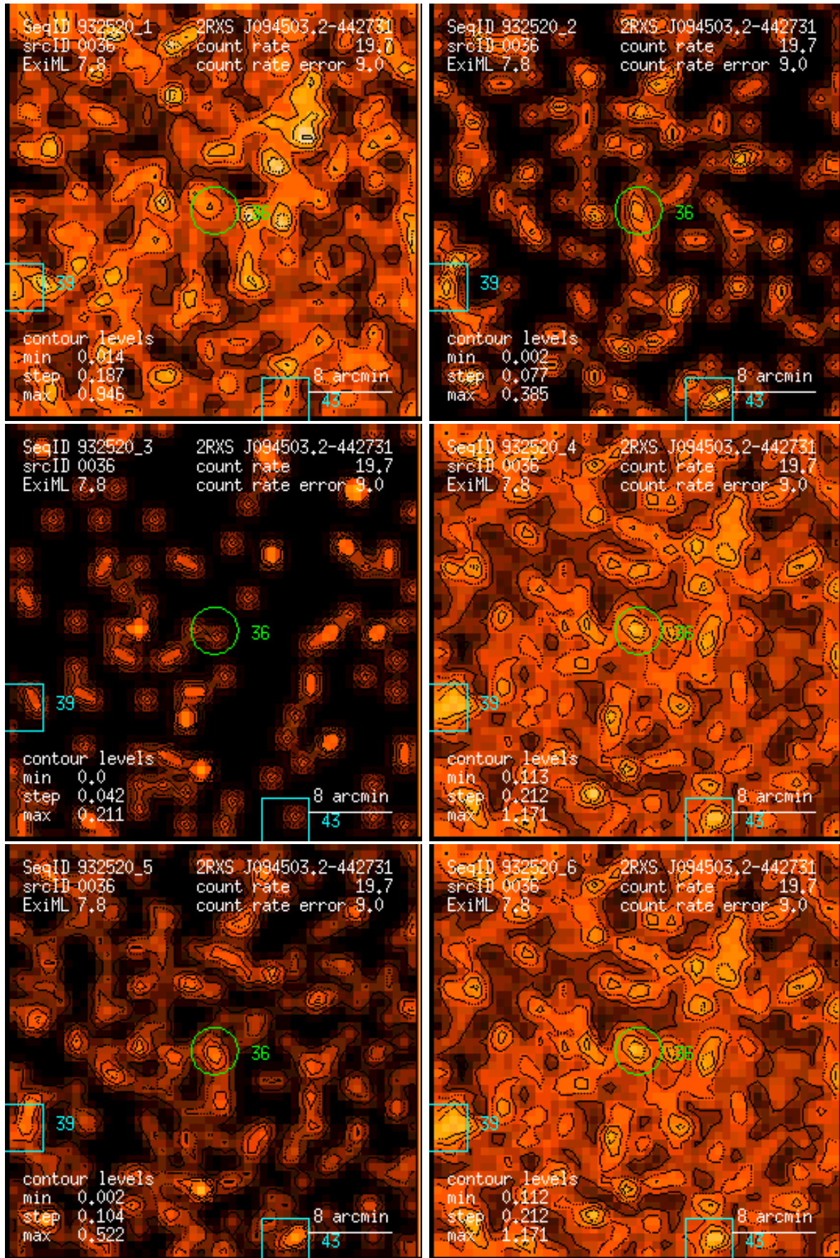
Figure 36: RASS 932520: detection 0036: band rate images, Gaussian filter: (1) PSPC channels 11 – 41, (2) 52 – 90, (3) 91 – 201, (4) 11 – 235, (5) 52 – 201, (6) 11 – 201. Broad band rates in counts/ks. Band rate contour levels in counts/ks/arcmin 2 .
