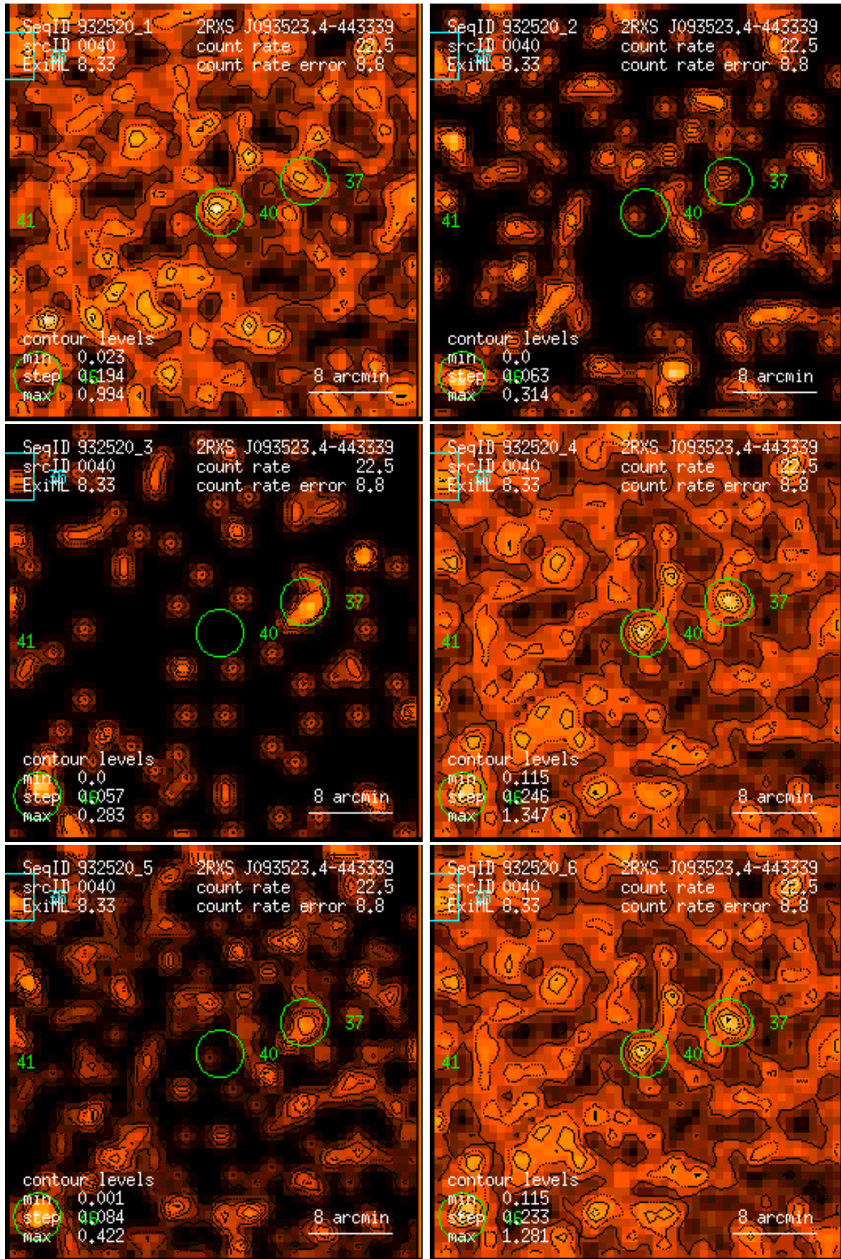
Figure 40: RASS 932520: detection 0040: band rate images, Gaussian filter: (1) PSPC channels 11 – 41, (2) 52 – 90, (3) 91 – 201, (4) 11 – 235, (5) 52 – 201, (6) 11 – 201. Broad band rates in counts/ks. Band rate contour levels in counts/ks/arcmin 2 .
