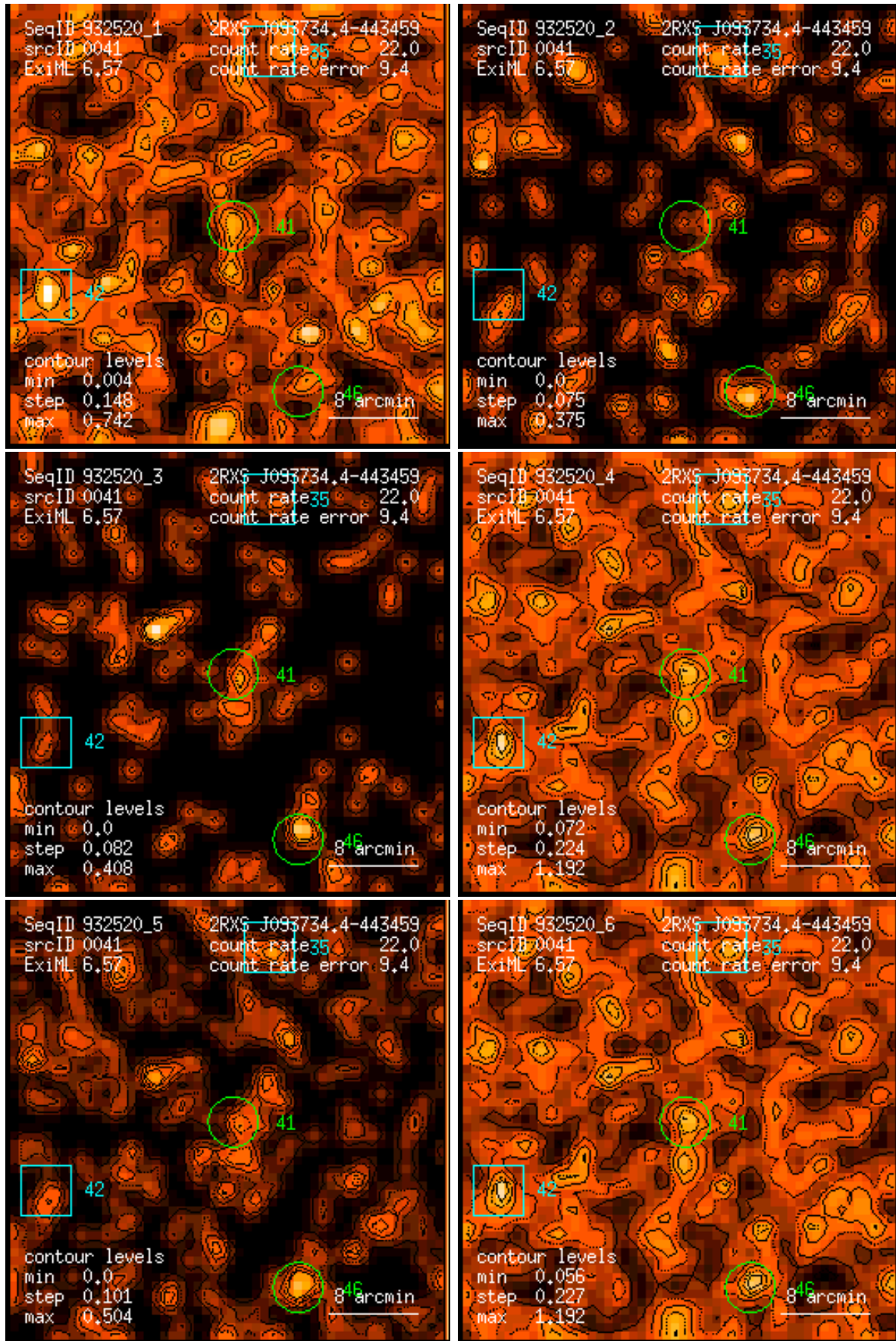
Figure 41: RASS 932520: detection 0041: band rate images, Gaussian filter: (1) PSPC channels 11 – 41, (2) 52 – 90, (3) 91 – 201, (4) 11 – 235, (5) 52 – 201, (6) 11 – 201. Broad band rates in counts/ks. Band rate contour levels in counts/ks/arcmin 2 .
