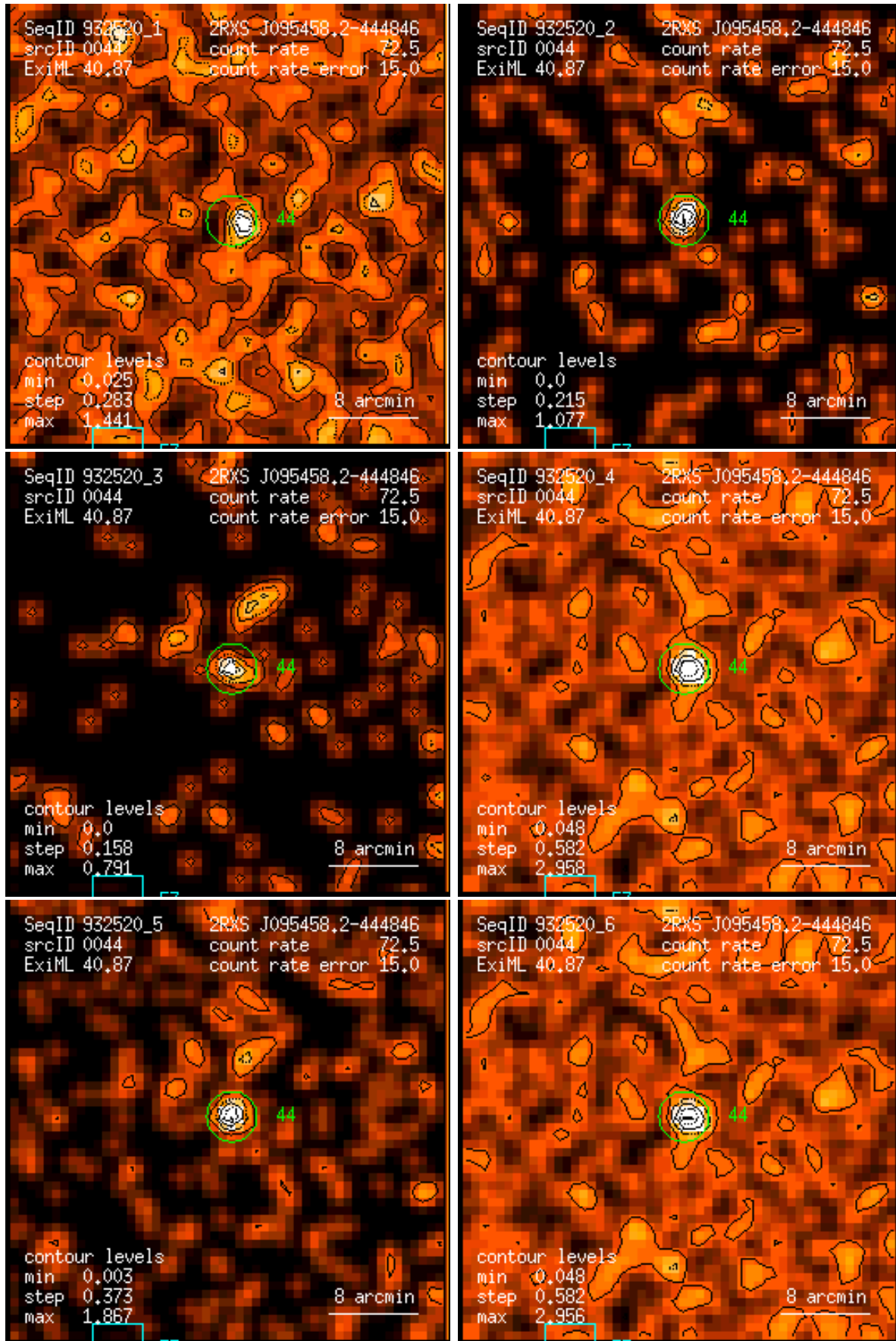
Figure 44: RASS 932520: detection 0044: band rate images, Gaussian filter: (1) PSPC channels 11 – 41, (2) 52 – 90, (3) 91 – 201, (4) 11 – 235, (5) 52 – 201, (6) 11 – 201. Broad band rates in counts/ks. Band rate contour levels in counts/ks/arcmin 2 .
