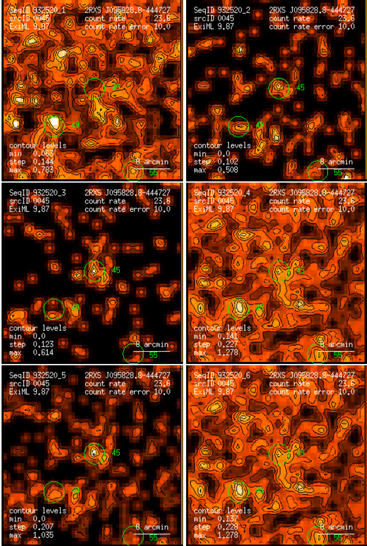
Figure 45: RASS 932520: detection 0045: band rate images, Gaussian filter: (1) PSPC channels 11 – 41, (2) 52 – 90, (3) 91 – 201, (4) 11 – 235, (5) 52 – 201, (6) 11 – 201. Broad band rates in counts/ks. Band rate contour levels in counts/ks/arcmin 2 .
