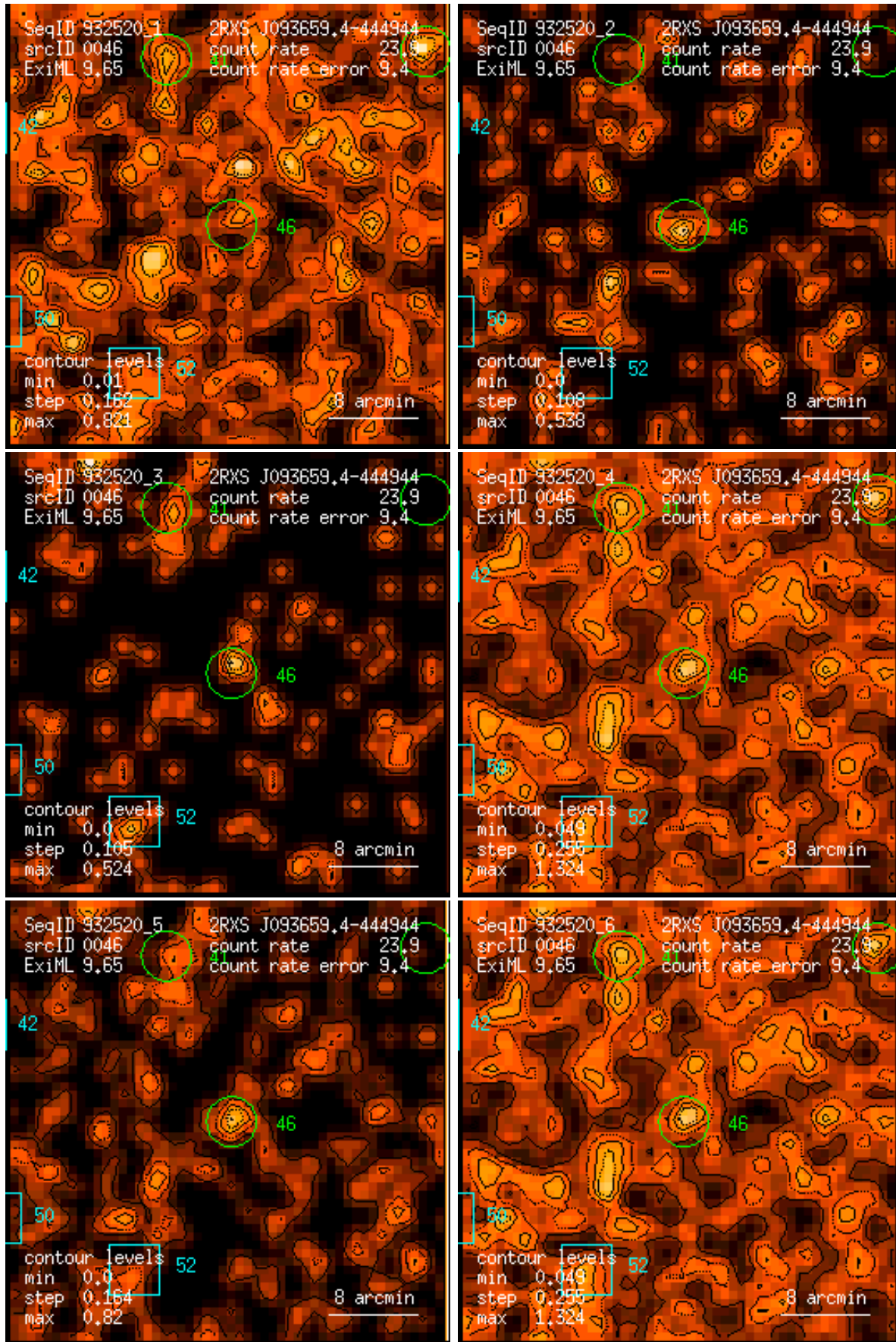
Figure 46: RASS 932520: detection 0046: band rate images, Gaussian filter: (1) PSPC channels 11 – 41, (2) 52 – 90, (3) 91 – 201, (4) 11 – 235, (5) 52 – 201, (6) 11 – 201. Broad band rates in counts/ks. Band rate contour levels in counts/ks/arcmin 2 .
