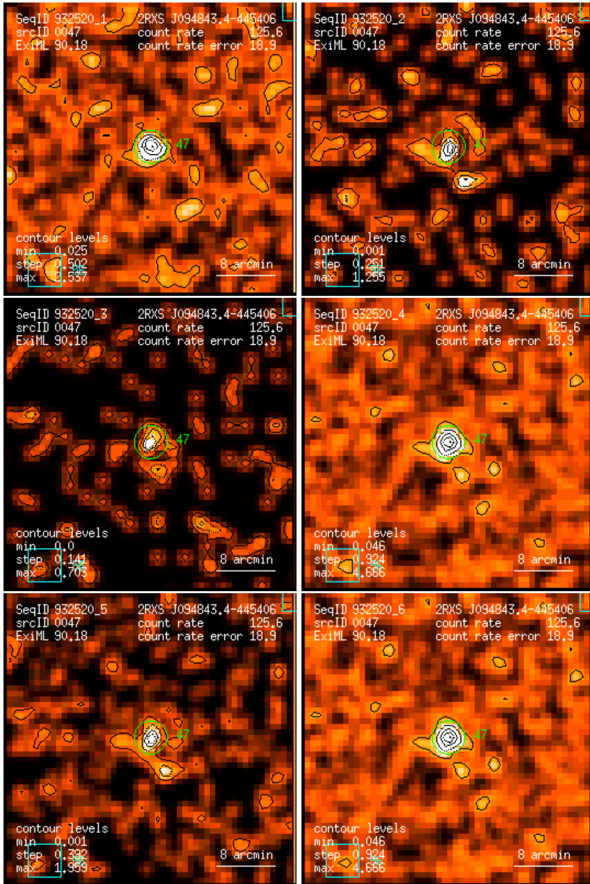
Figure 47: RASS 932520: detection 0047: band rate images, Gaussian filter: (1) PSPC channels 11 – 41, (2) 52 – 90, (3) 91 – 201, (4) 11 – 235, (5) 52 – 201, (6) 11 – 201. Broad band rates in counts/ks. Band rate contour levels in counts/ks/arcmin 2 .
