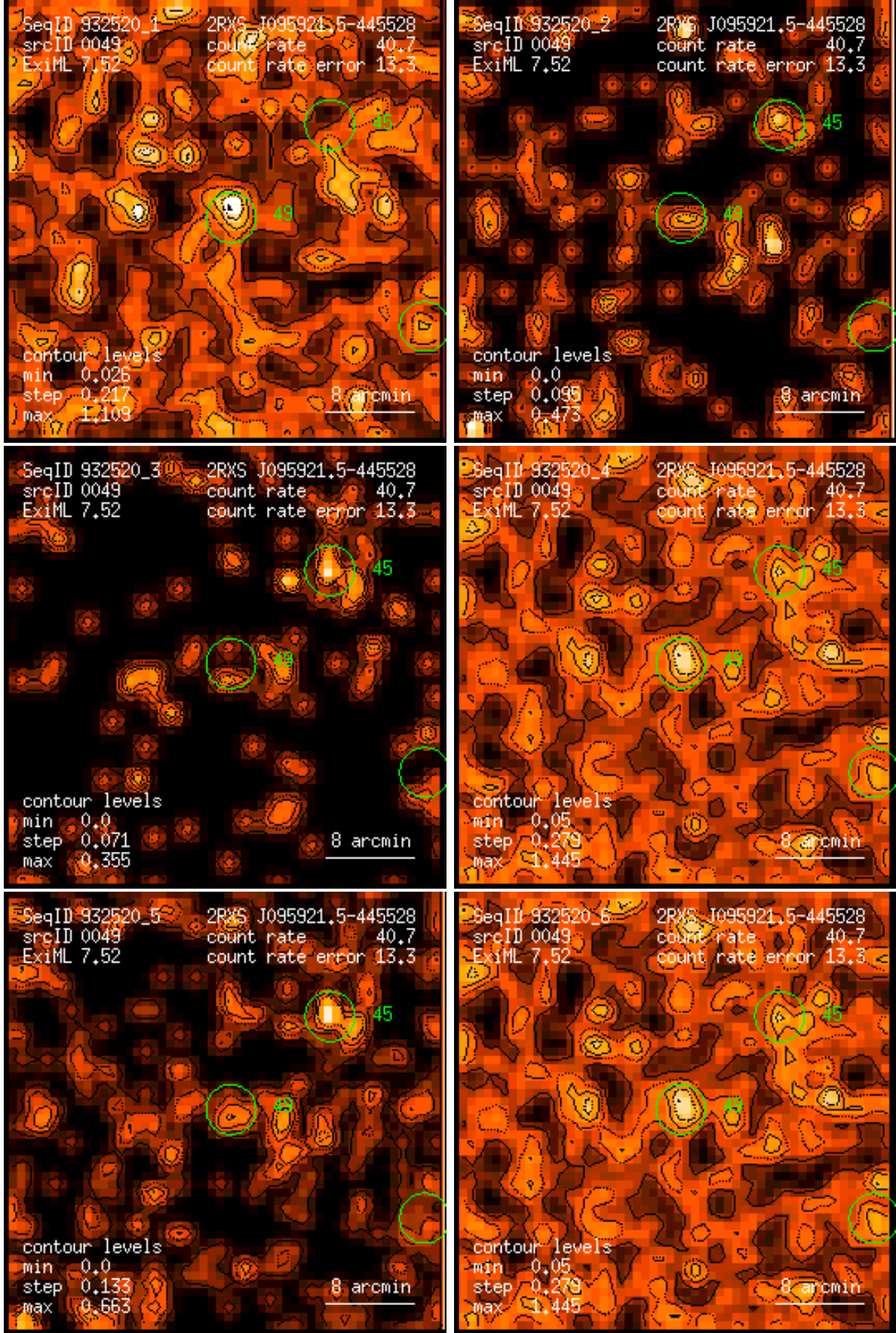
Figure 49: RASS 932520: detection 0049: band rate images, Gaussian filter: (1) PSPC channels 11 – 41, (2) 52 – 90, (3) 91 – 201, (4) 11 – 235, (5) 52 – 201, (6) 11 – 201. Broad band rates in counts/ks. Band rate contour levels in counts/ks/arcmin 2 .
