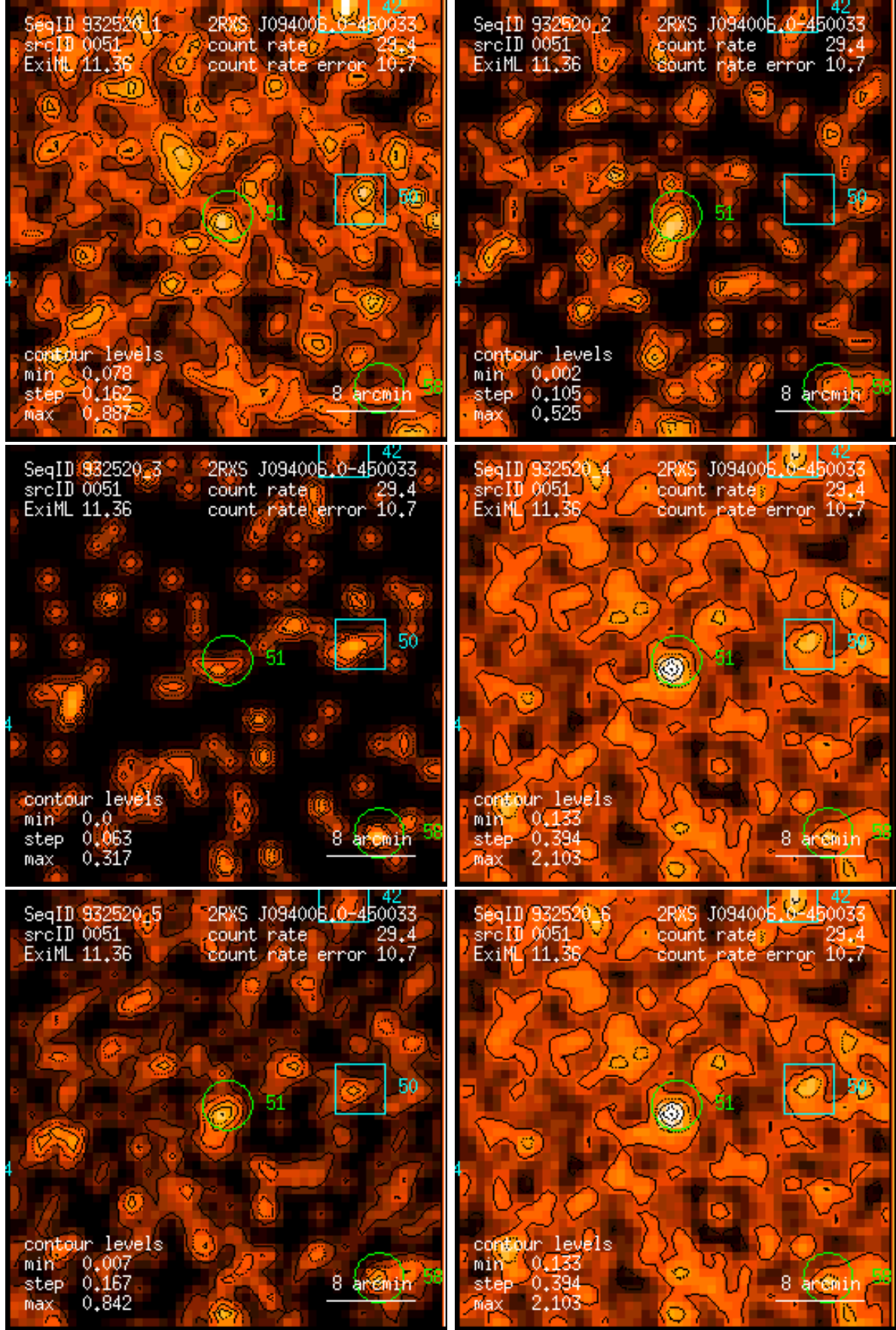
Figure 51: RASS 932520: detection 0051: band rate images, Gaussian filter: (1) PSPC channels 11 – 41, (2) 52 – 90, (3) 91 – 201, (4) 11 – 235, (5) 52 – 201, (6) 11 – 201. Broad band rates in counts/ks. Band rate contour levels in counts/ks/arcmin 2 .
