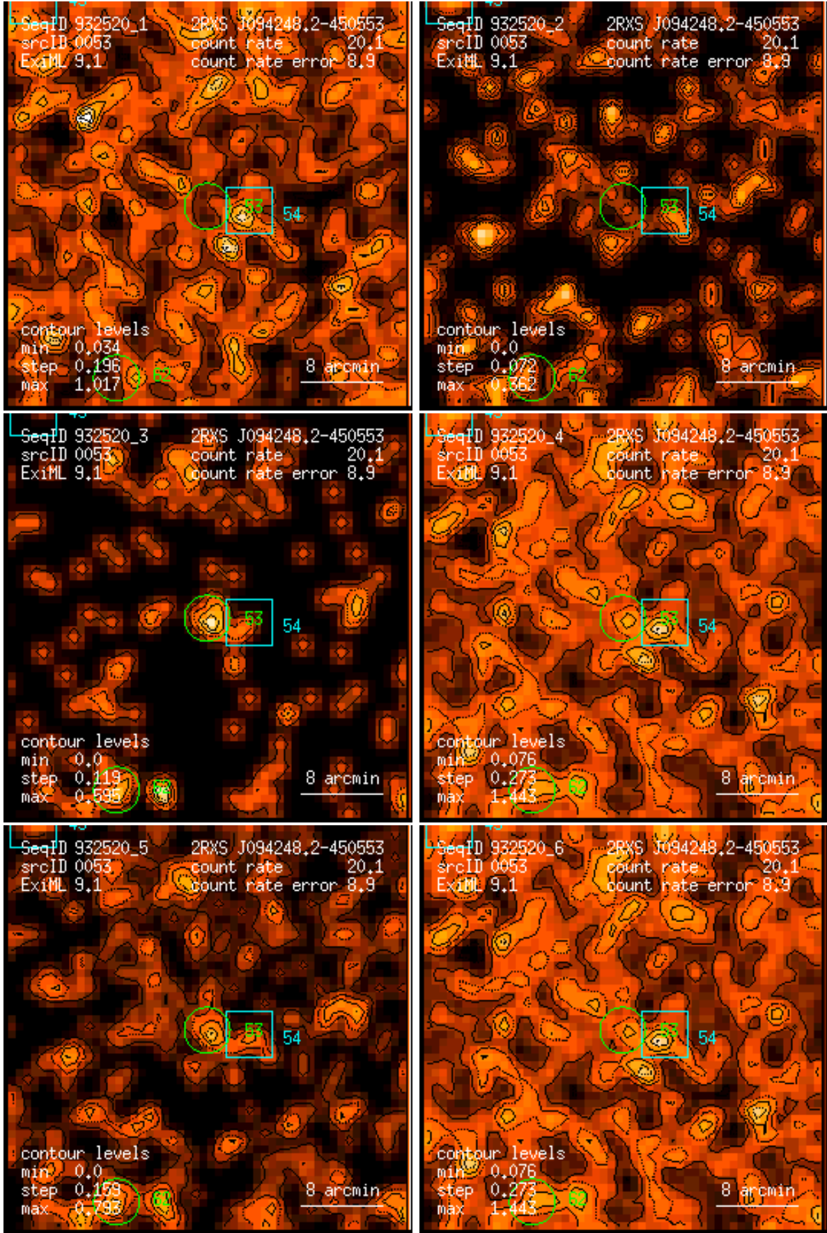
Figure 53: RASS 932520: detection 0053: band rate images, Gaussian filter: (1) PSPC channels 11 – 41, (2) 52 – 90, (3) 91 – 201, (4) 11 – 235, (5) 52 – 201, (6) 11 – 201. Broad band rates in counts/ks. Band rate contour levels in counts/ks/arcmin 2 .
