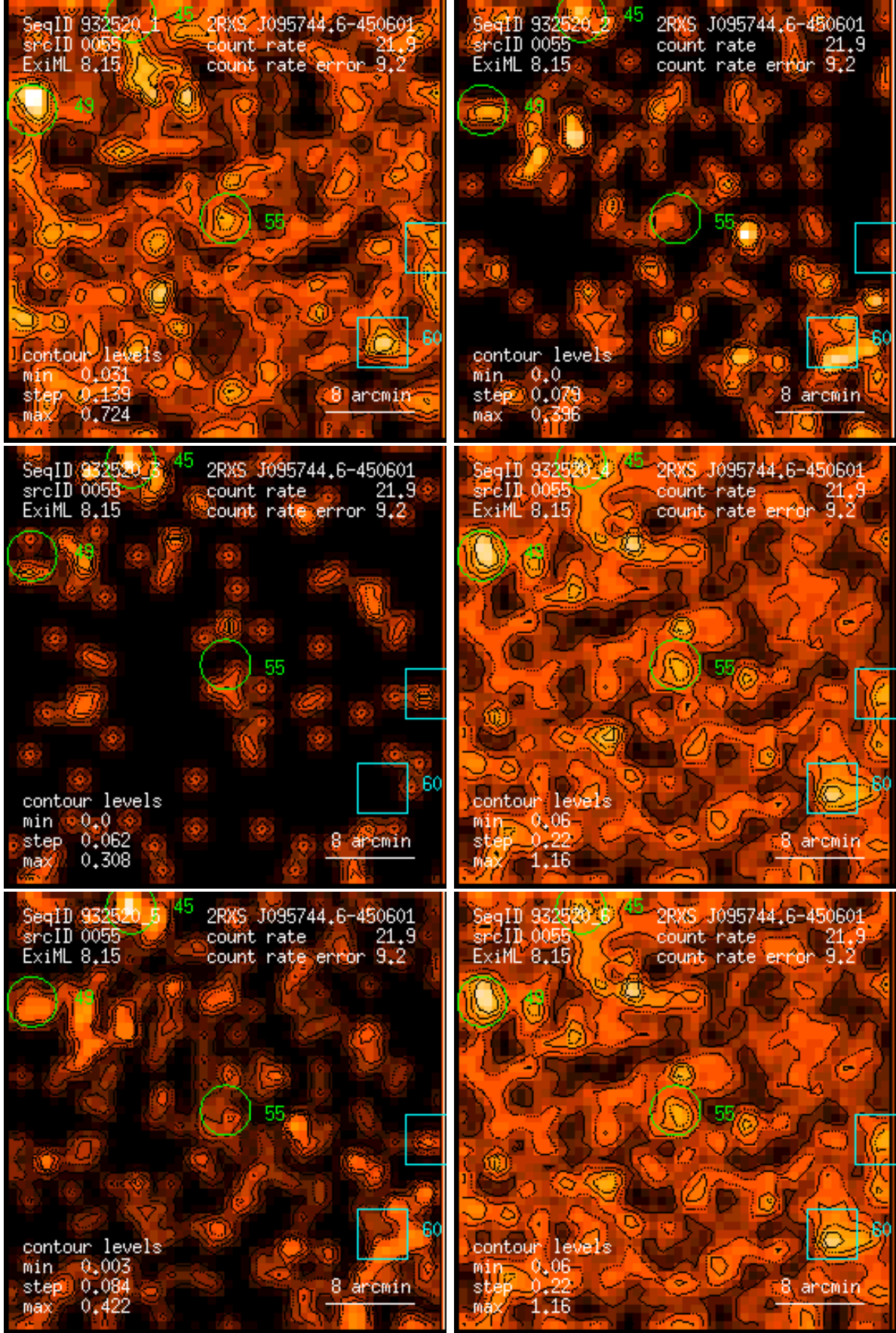
Figure 55: RASS 932520: detection 0055: band rate images, Gaussian filter: (1) PSPC channels 11 – 41, (2) 52 – 90, (3) 91 – 201, (4) 11 – 235, (5) 52 – 201, (6) 11 – 201. Broad band rates in counts/ks. Band rate contour levels in counts/ks/arcmin 2 .
